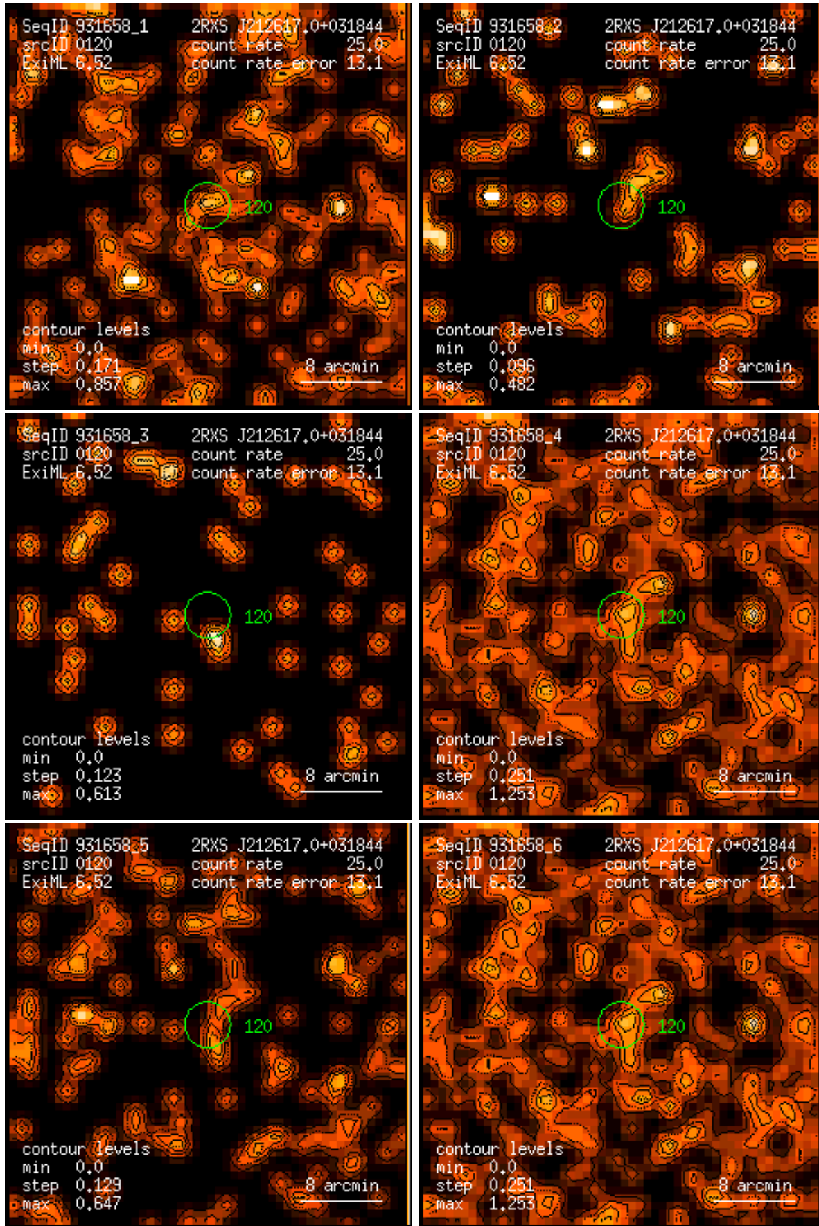
Figure 120: RASS 931658: detection 0120: band rate images, Gaussian filter: (1) PSPC channels 11 – 41, (2) 52 – 90, (3) 91 – 201, (4) 11 – 235, (5) 52 – 201, (6) 11 – 201. Broad band rates in counts/ks. Band rate contour levels in counts/ks/arcmin 2 .
