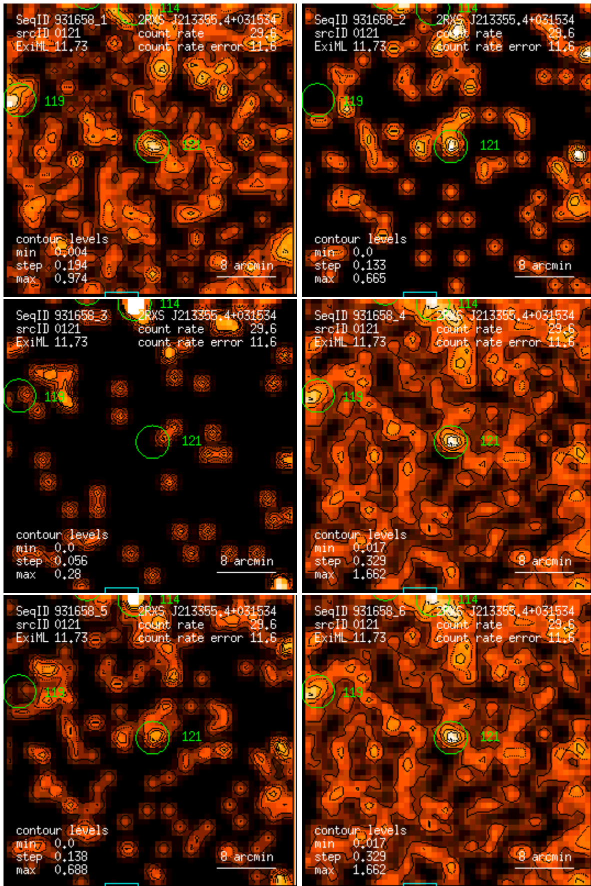
Figure 121: RASS 931658: detection 0121: band rate images, Gaussian filter: (1) PSPC channels 11 – 41, (2) 52 – 90, (3) 91 – 201, (4) 11 – 235, (5) 52 – 201, (6) 11 – 201. Broad band rates in counts/ks. Band rate contour levels in counts/ks/arcmin 2 .
