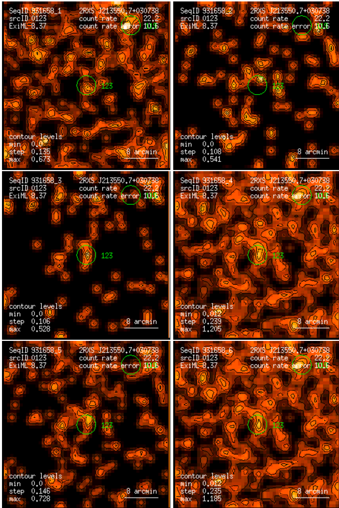
Figure 123: RASS 931658: detection 0123: band rate images, Gaussian filter: (1) PSPC channels 11 – 41, (2) 52 – 90, (3) 91 – 201, (4) 11 – 235, (5) 52 – 201, (6) 11 – 201. Broad band rates in counts/ks. Band rate contour levels in counts/ks/arcmin 2 .
