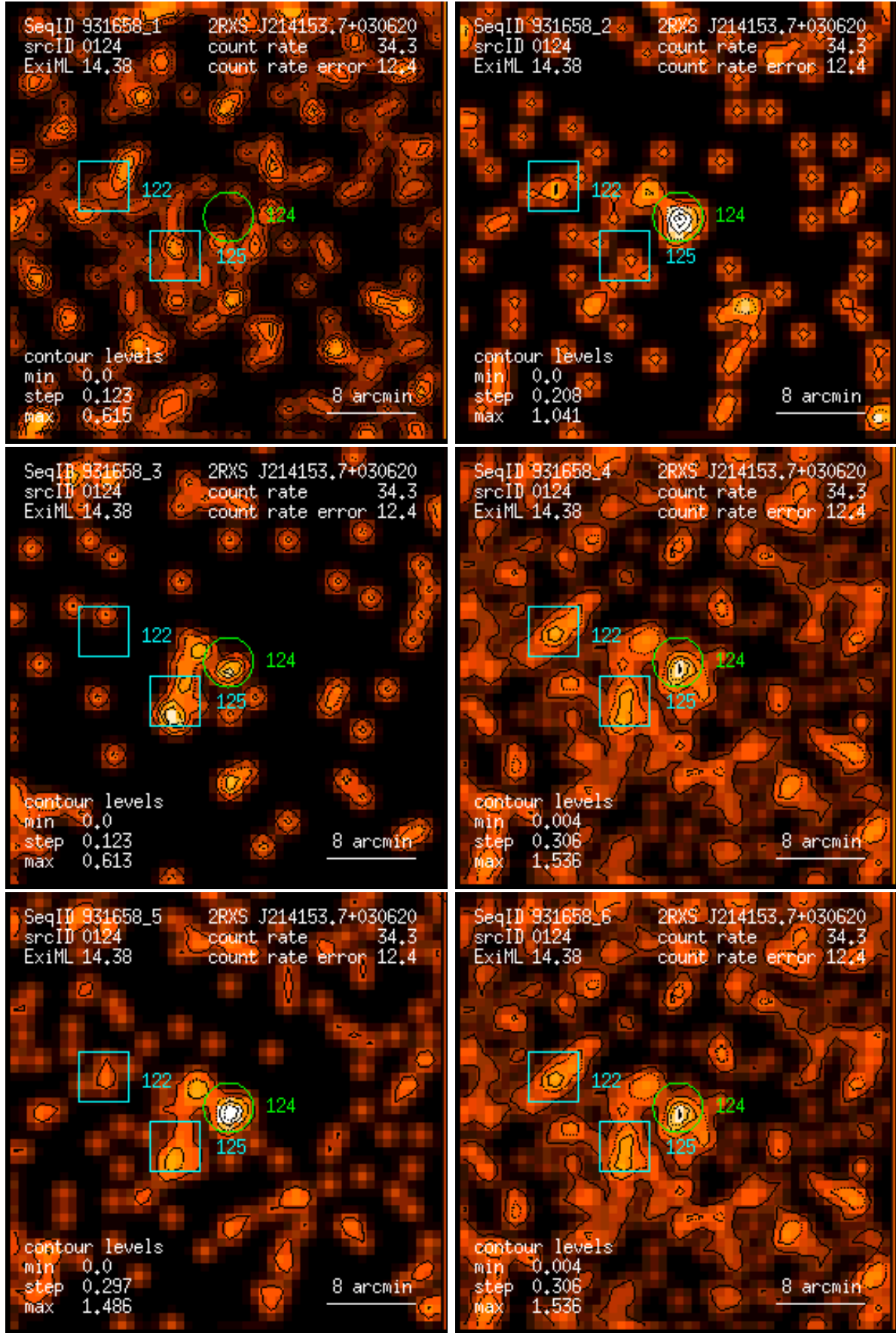
Figure 124: RASS 931658: detection 0124: band rate images, Gaussian filter: (1) PSPC channels 11 – 41, (2) 52 – 90, (3) 91 – 201, (4) 11 – 235, (5) 52 – 201, (6) 11 – 201. Broad band rates in counts/ks. Band rate contour levels in counts/ks/arcmin 2 .
