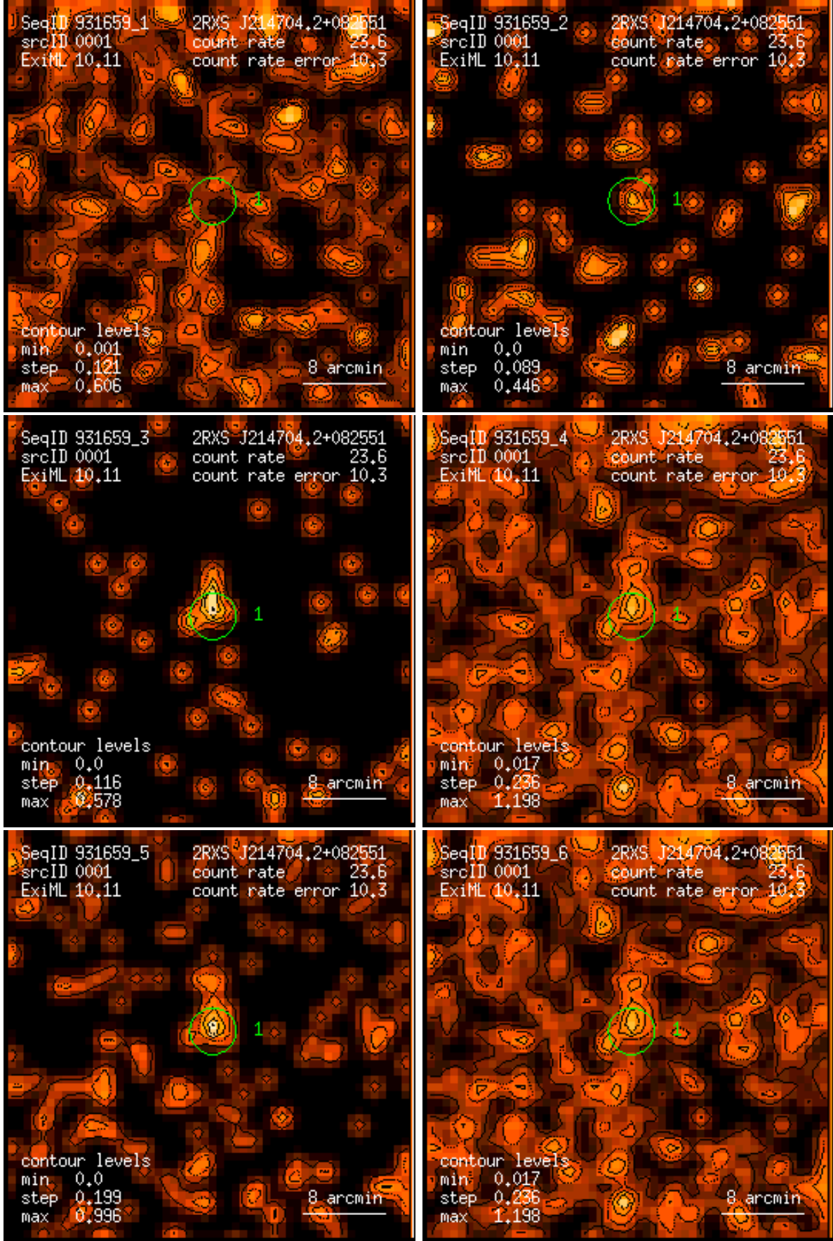
Figure 1: RASS 931659: detection 0001: band rate images, Gaussian filter: (1) PSPC channels 11 – 41, (2) 52 – 90, (3) 91 – 201, (4) 11 – 235, (5) 52 – 201, (6) 11 – 201. Broad band rates in counts/ks. Band rate contour levels in counts/ks/arcmin 2 .
