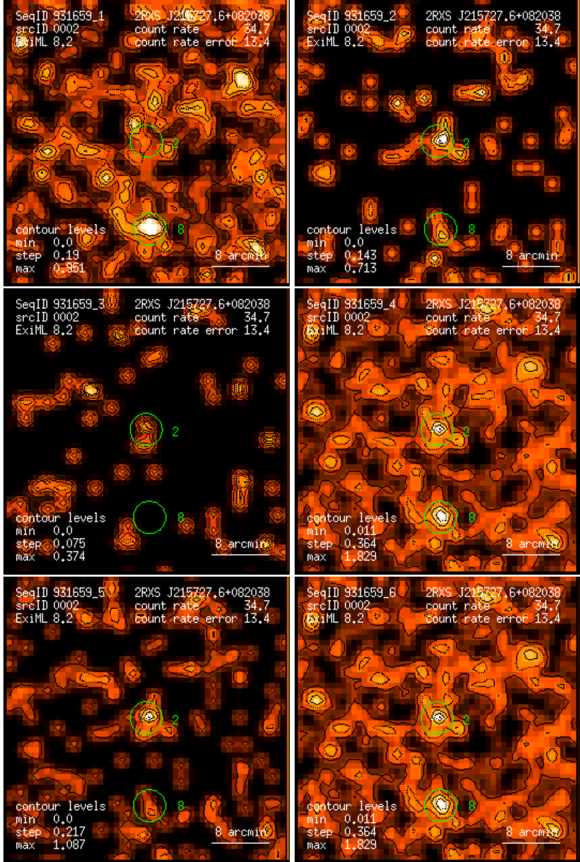
Figure 2: RASS 931659: detection 0002: band rate images, Gaussian filter: (1) PSPC channels 11 – 41, (2) 52 – 90, (3) 91 – 201, (4) 11 – 235, (5) 52 – 201, (6) 11 – 201. Broad band rates in counts/ks. Band rate contour levels in counts/ks/arcmin 2 .
