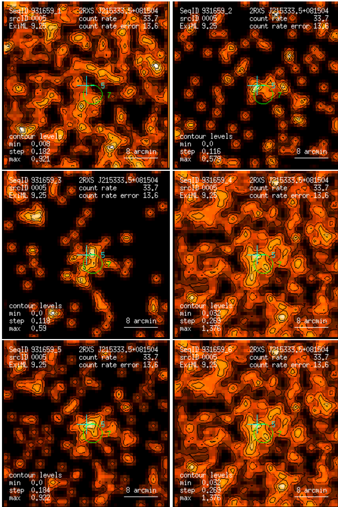
Figure 5: RASS 931659: detection 0005: band rate images, Gaussian filter: (1) PSPC channels 11 – 41, (2) 52 – 90, (3) 91 – 201, (4) 11 – 235, (5) 52 – 201, (6) 11 – 201. Broad band rates in counts/ks. Band rate contour levels in counts/ks/arcmin 2 .
