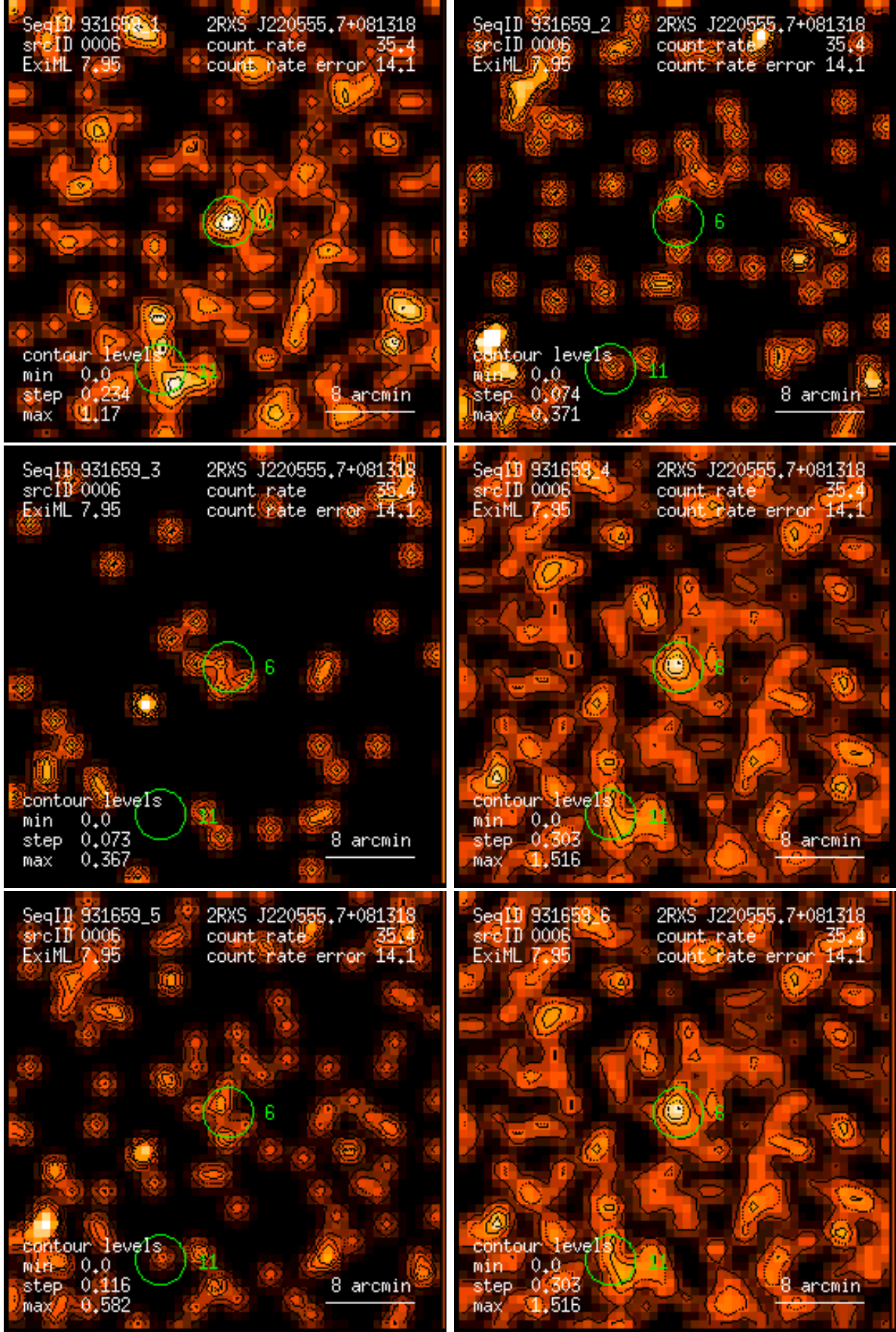
Figure 6: RASS 931659: detection 0006: band rate images, Gaussian filter: (1) PSPC channels 11 – 41, (2) 52 – 90, (3) 91 – 201, (4) 11 – 235, (5) 52 – 201, (6) 11 – 201. Broad band rates in counts/ks. Band rate contour levels in counts/ks/arcmin 2 .
