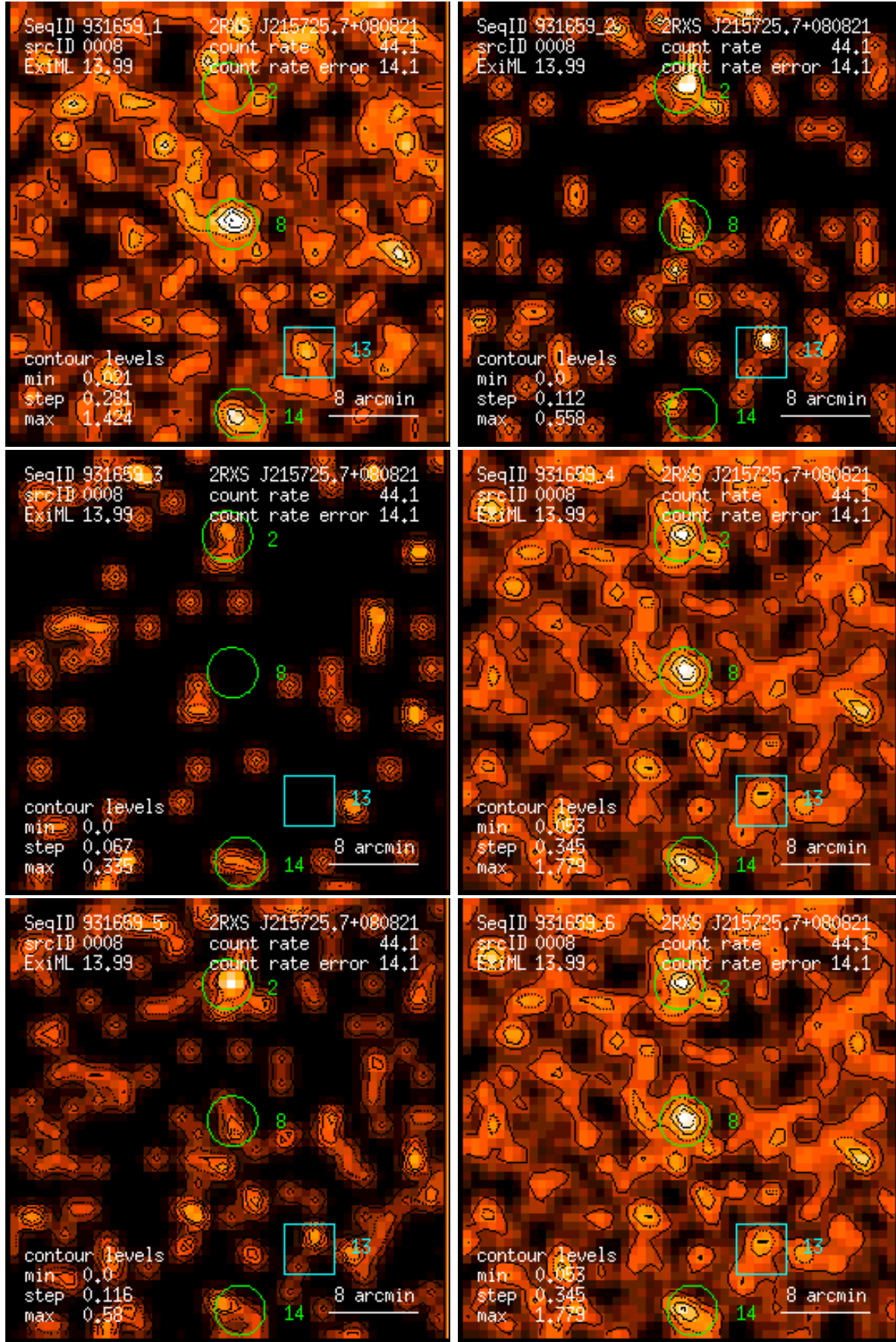
Figure 8: RASS 931659: detection 0008: band rate images, Gaussian filter: (1) PSPC channels 11 – 41, (2) 52 – 90, (3) 91 – 201, (4) 11 – 235, (5) 52 – 201, (6) 11 – 201. Broad band rates in counts/ks. Band rate contour levels in counts/ks/arcmin 2 .
