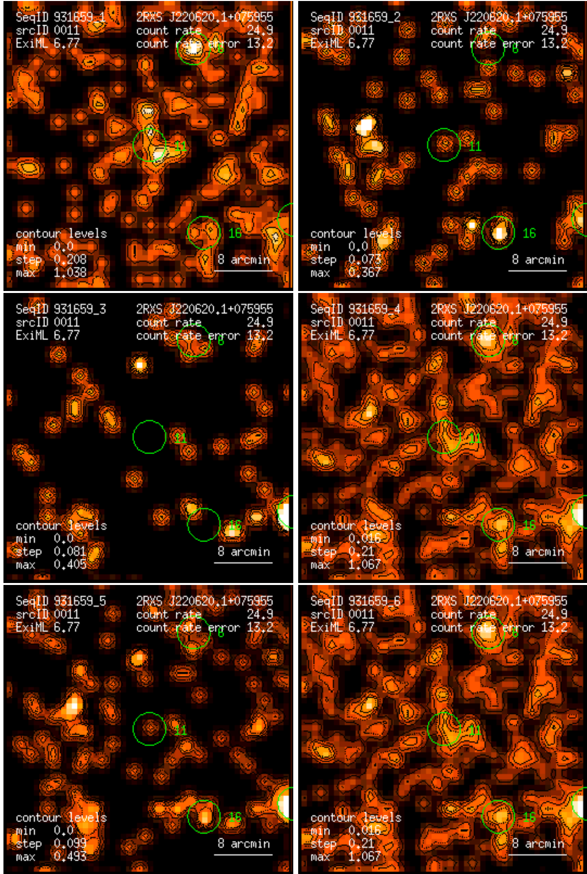
Figure 11: RASS 931659: detection 0011: band rate images, Gaussian filter: (1) PSPC channels 11 – 41, (2) 52 – 90, (3) 91 – 201, (4) 11 – 235, (5) 52 – 201, (6) 11 – 201. Broad band rates in counts/ks. Band rate contour levels in counts/ks/arcmin 2 .
