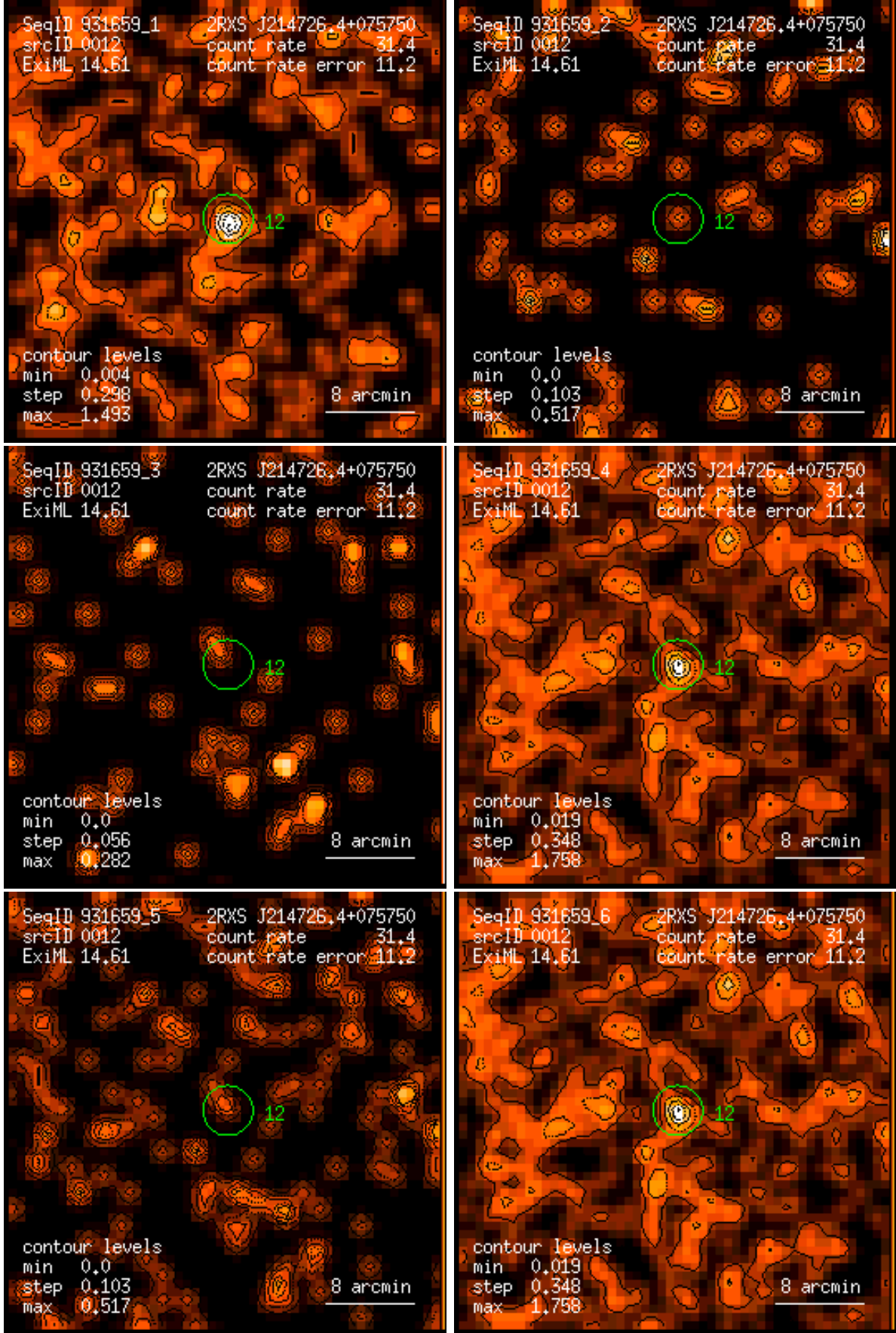
Figure 12: RASS 931659: detection 0012: band rate images, Gaussian filter: (1) PSPC channels 11 – 41, (2) 52 – 90, (3) 91 – 201, (4) 11 – 235, (5) 52 – 201, (6) 11 – 201. Broad band rates in counts/ks. Band rate contour levels in counts/ks/arcmin 2 .
