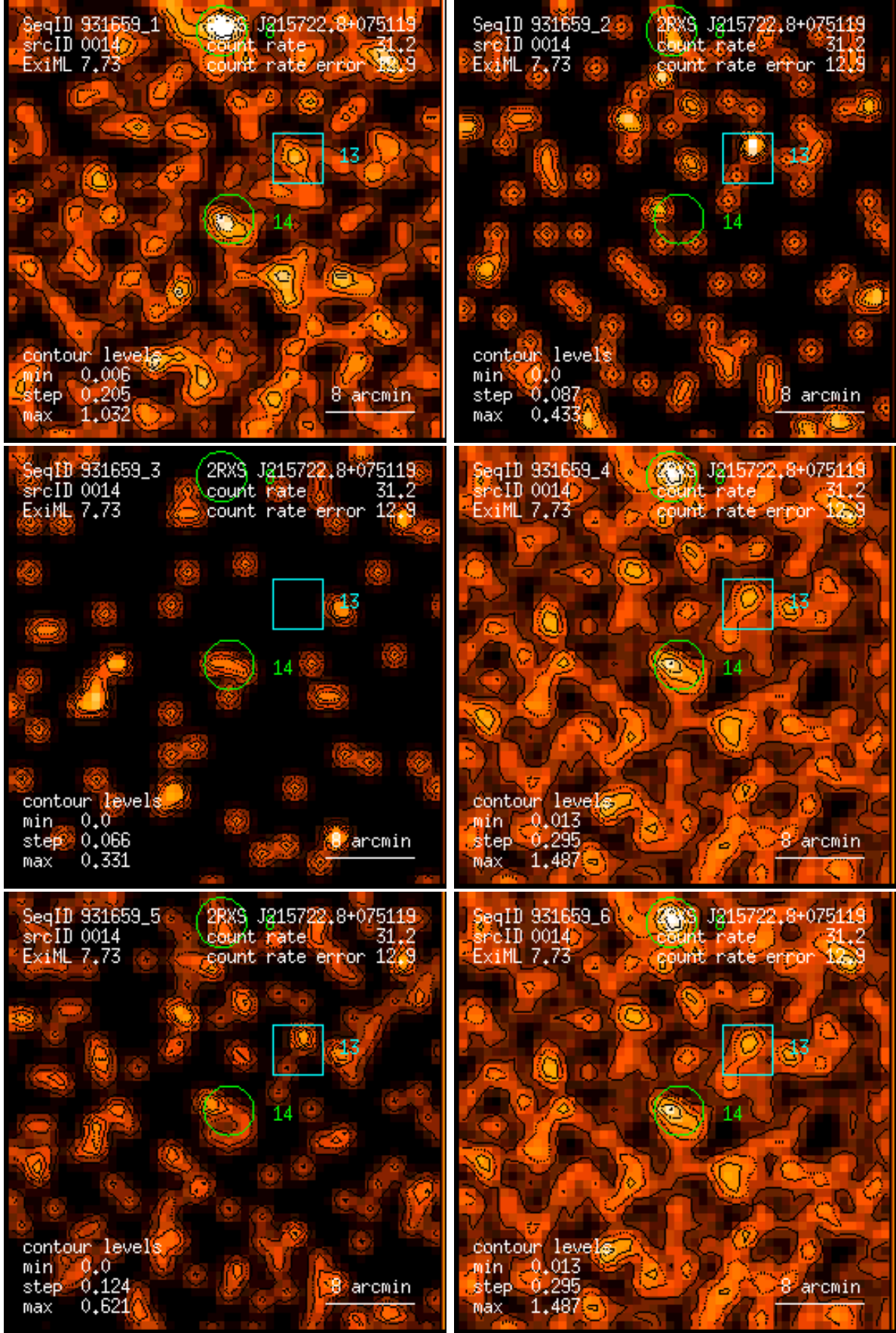
Figure 14: RASS 931659: detection 0014: band rate images, Gaussian filter: (1) PSPC channels 11 – 41, (2) 52 – 90, (3) 91 – 201, (4) 11 – 235, (5) 52 – 201, (6) 11 – 201. Broad band rates in counts/ks. Band rate contour levels in counts/ks/arcmin 2 .
