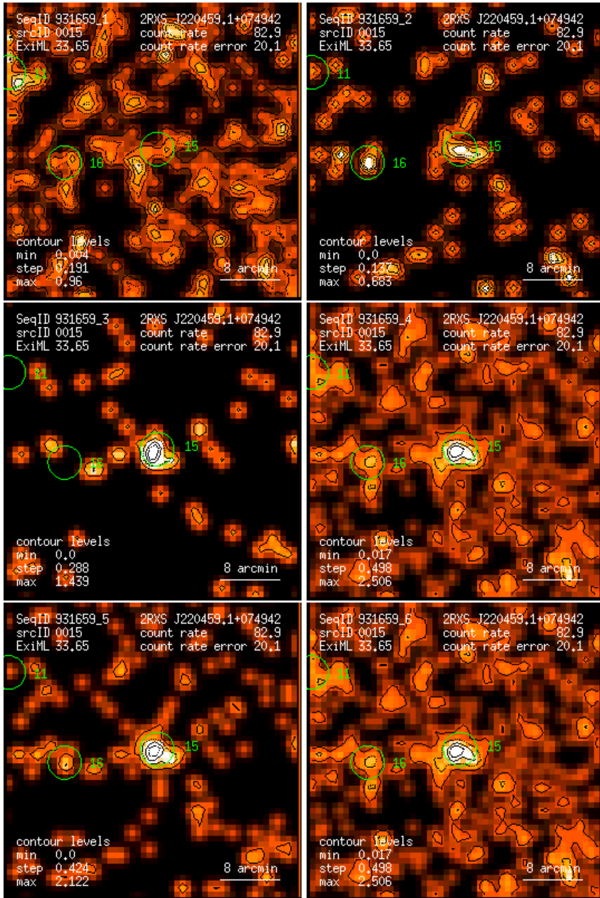
Figure 15: RASS 931659: detection 0015: band rate images, Gaussian filter: (1) PSPC channels 11 – 41, (2) 52 – 90, (3) 91 – 201, (4) 11 – 235, (5) 52 – 201, (6) 11 – 201. Broad band rates in counts/ks. Band rate contour levels in counts/ks/arcmin 2 .
