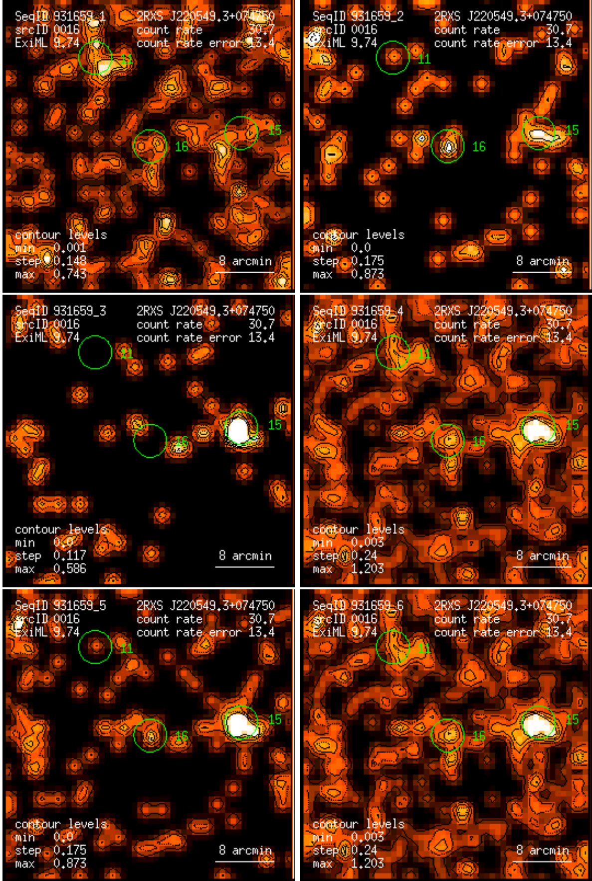
Figure 16: RASS 931659: detection 0016: band rate images, Gaussian filter: (1) PSPC channels 11 – 41, (2) 52 – 90, (3) 91 – 201, (4) 11 – 235, (5) 52 – 201, (6) 11 – 201. Broad band rates in counts/ks. Band rate contour levels in counts/ks/arcmin 2 .
