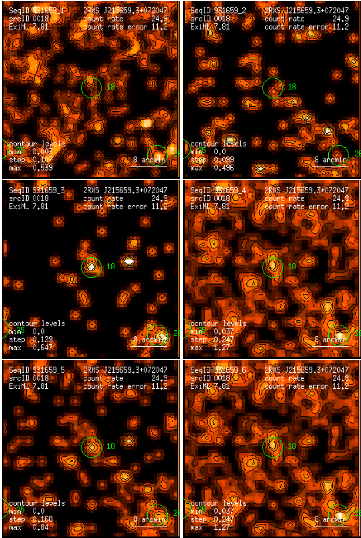
Figure 18: RASS 931659: detection 0018: band rate images, Gaussian filter: (1) PSPC channels 11 – 41, (2) 52 – 90, (3) 91 – 201, (4) 11 – 235, (5) 52 – 201, (6) 11 – 201. Broad band rates in counts/ks. Band rate contour levels in counts/ks/arcmin 2 .
