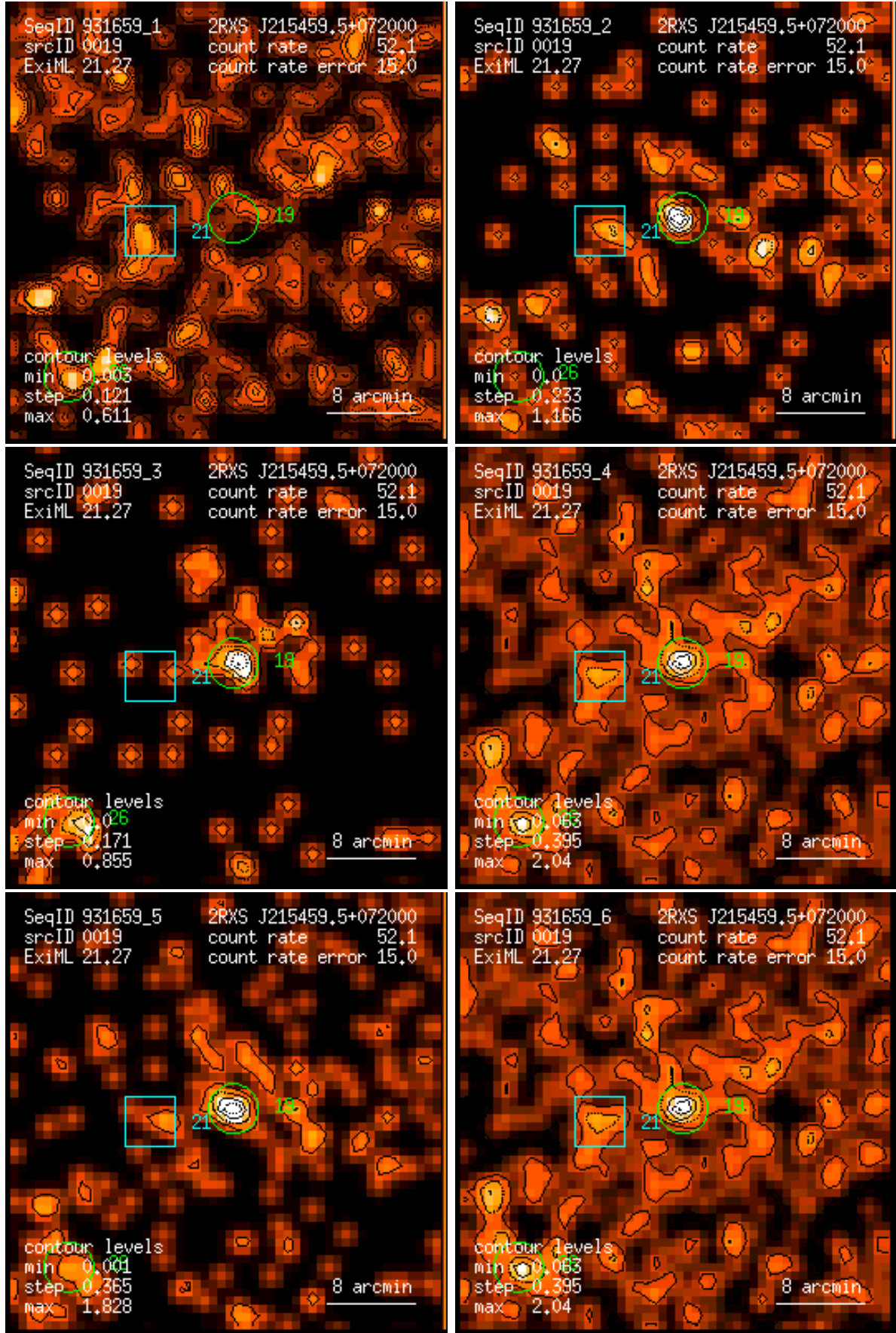
Figure 19: RASS 931659: detection 0019: band rate images, Gaussian filter: (1) PSPC channels 11 – 41, (2) 52 – 90, (3) 91 – 201, (4) 11 – 235, (5) 52 – 201, (6) 11 – 201. Broad band rates in counts/ks. Band rate contour levels in counts/ks/arcmin 2 .
