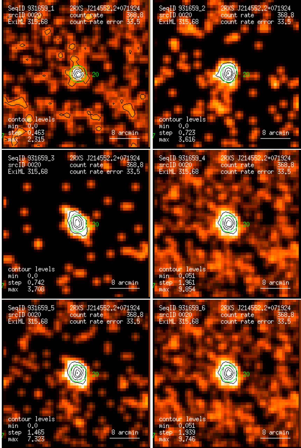
Figure 20: RASS 931659: detection 0020: band rate images, Gaussian filter: (1) PSPC channels 11 – 41, (2) 52 – 90, (3) 91 – 201, (4) 11 – 235, (5) 52 – 201, (6) 11 – 201. Broad band rates in counts/ks. Band rate contour levels in counts/ks/arcmin 2 .
