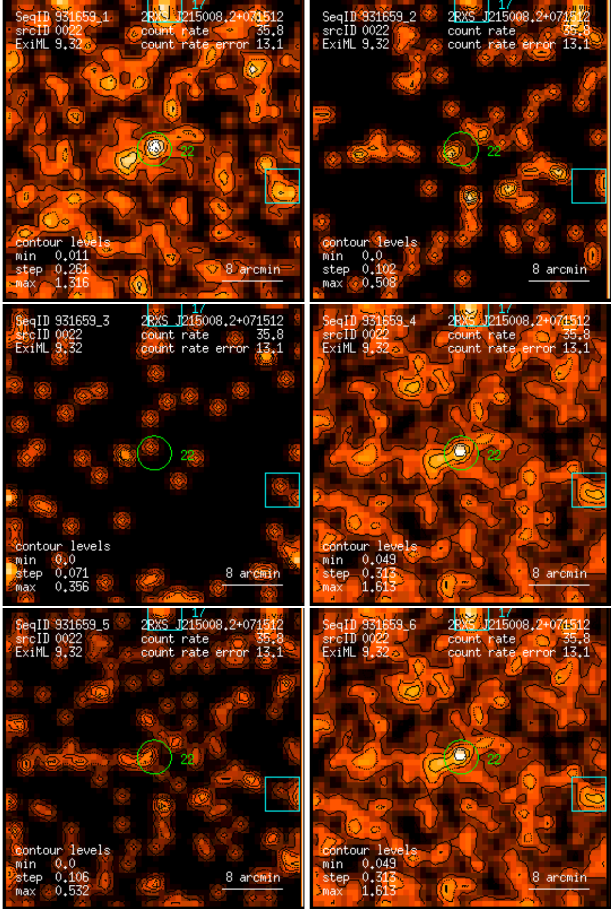
Figure 22: RASS 931659: detection 0022: band rate images, Gaussian filter: (1) PSPC channels 11 – 41, (2) 52 – 90, (3) 91 – 201, (4) 11 – 235, (5) 52 – 201, (6) 11 – 201. Broad band rates in counts/ks. Band rate contour levels in counts/ks/arcmin 2 .
