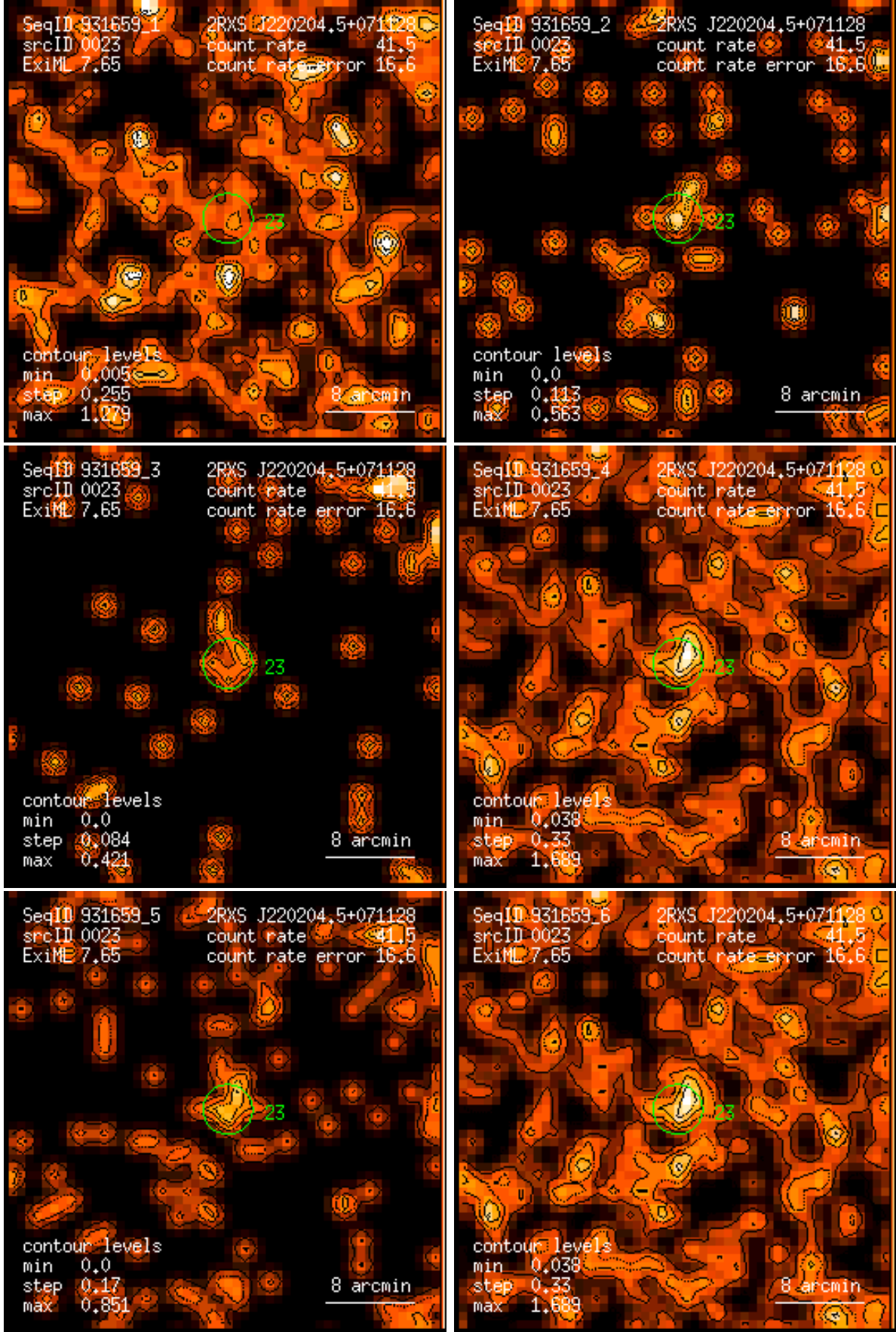
Figure 23: RASS 931659: detection 0023: band rate images, Gaussian filter: (1) PSPC channels 11 – 41, (2) 52 – 90, (3) 91 – 201, (4) 11 – 235, (5) 52 – 201, (6) 11 – 201. Broad band rates in counts/ks. Band rate contour levels in counts/ks/arcmin 2 .
