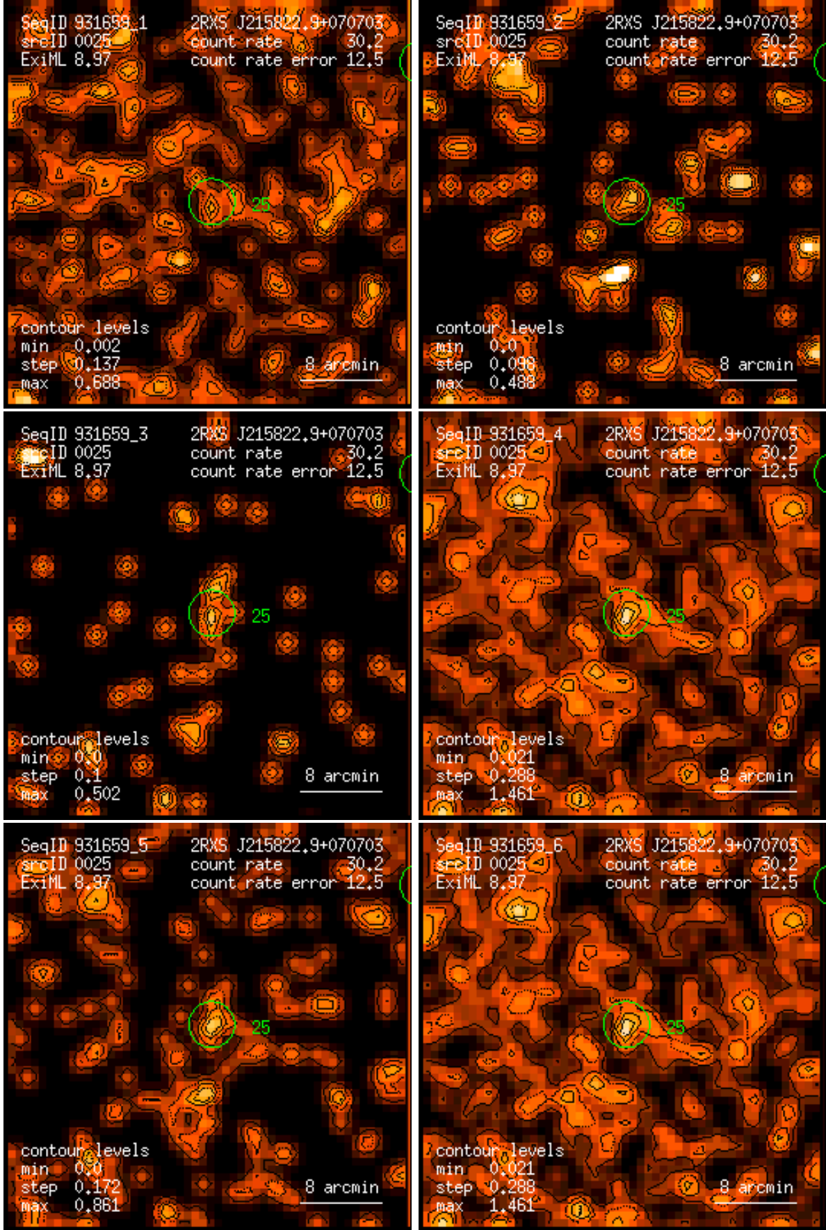
Figure 25: RASS 931659: detection 0025: band rate images, Gaussian filter: (1) PSPC channels 11 – 41, (2) 52 – 90, (3) 91 – 201, (4) 11 – 235, (5) 52 – 201, (6) 11 – 201. Broad band rates in counts/ks. Band rate contour levels in counts/ks/arcmin 2 .
