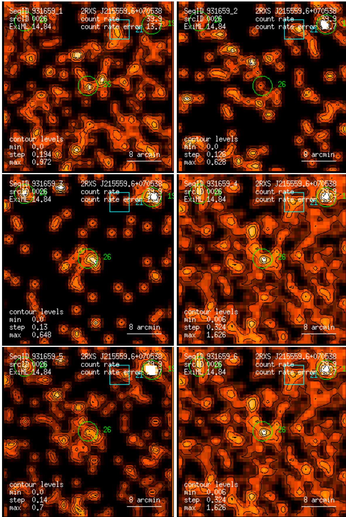
Figure 26: RASS 931659: detection 0026: band rate images, Gaussian filter: (1) PSPC channels 11 – 41, (2) 52 – 90, (3) 91 – 201, (4) 11 – 235, (5) 52 – 201, (6) 11 – 201. Broad band rates in counts/ks. Band rate contour levels in counts/ks/arcmin 2 .
