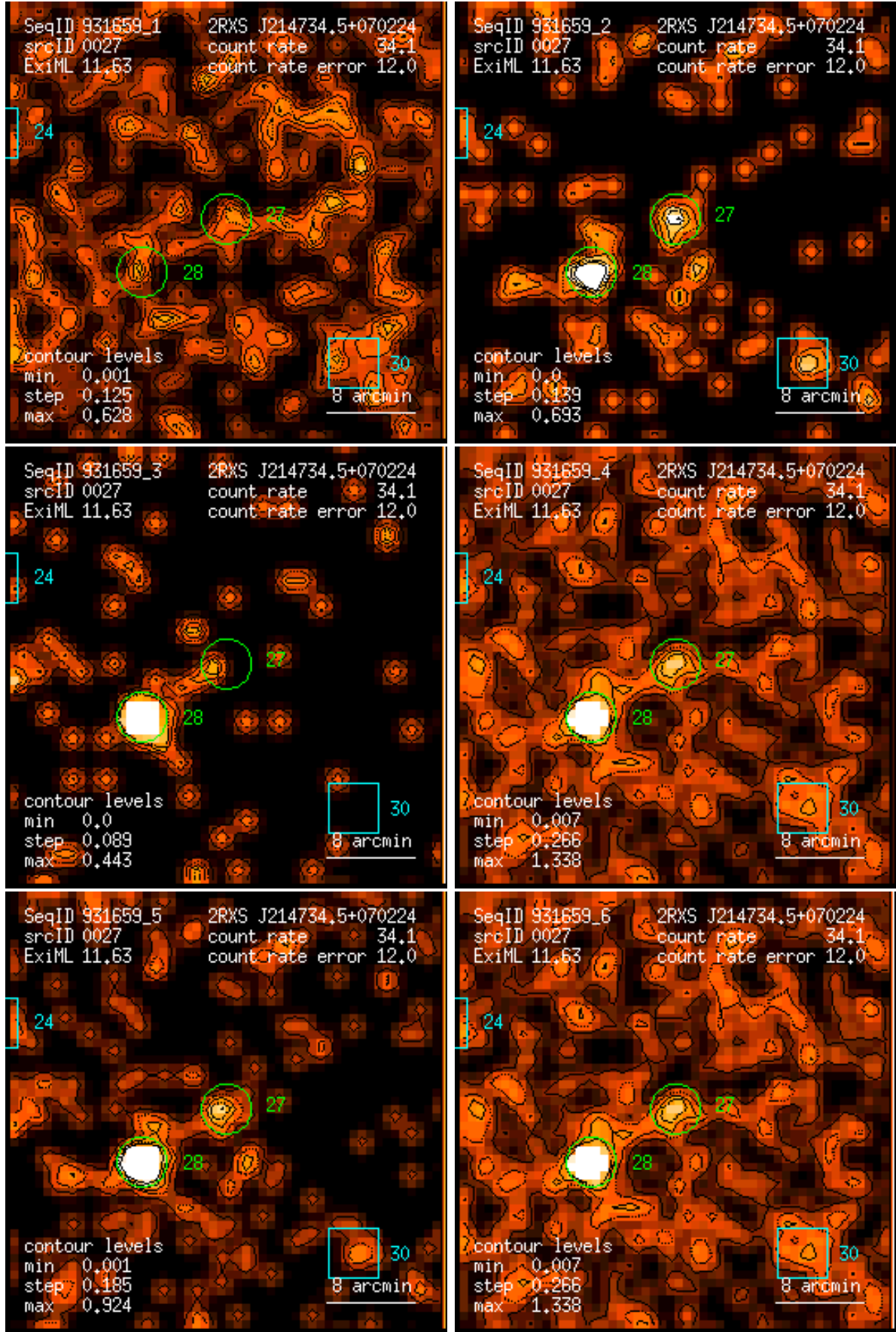
Figure 27: RASS 931659: detection 0027: band rate images, Gaussian filter: (1) PSPC channels 11 – 41, (2) 52 – 90, (3) 91 – 201, (4) 11 – 235, (5) 52 – 201, (6) 11 – 201. Broad band rates in counts/ks. Band rate contour levels in counts/ks/arcmin 2 .
