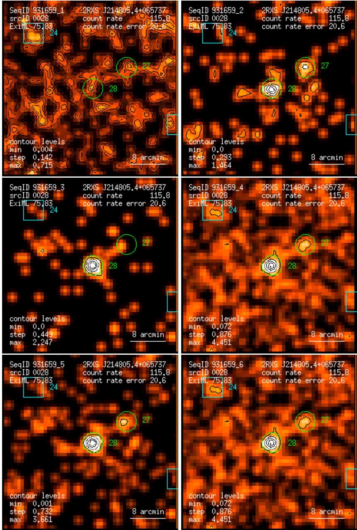
Figure 28: RASS 931659: detection 0028: band rate images, Gaussian filter: (1) PSPC channels 11 – 41, (2) 52 – 90, (3) 91 – 201, (4) 11 – 235, (5) 52 – 201, (6) 11 – 201. Broad band rates in counts/ks. Band rate contour levels in counts/ks/arcmin 2 .
