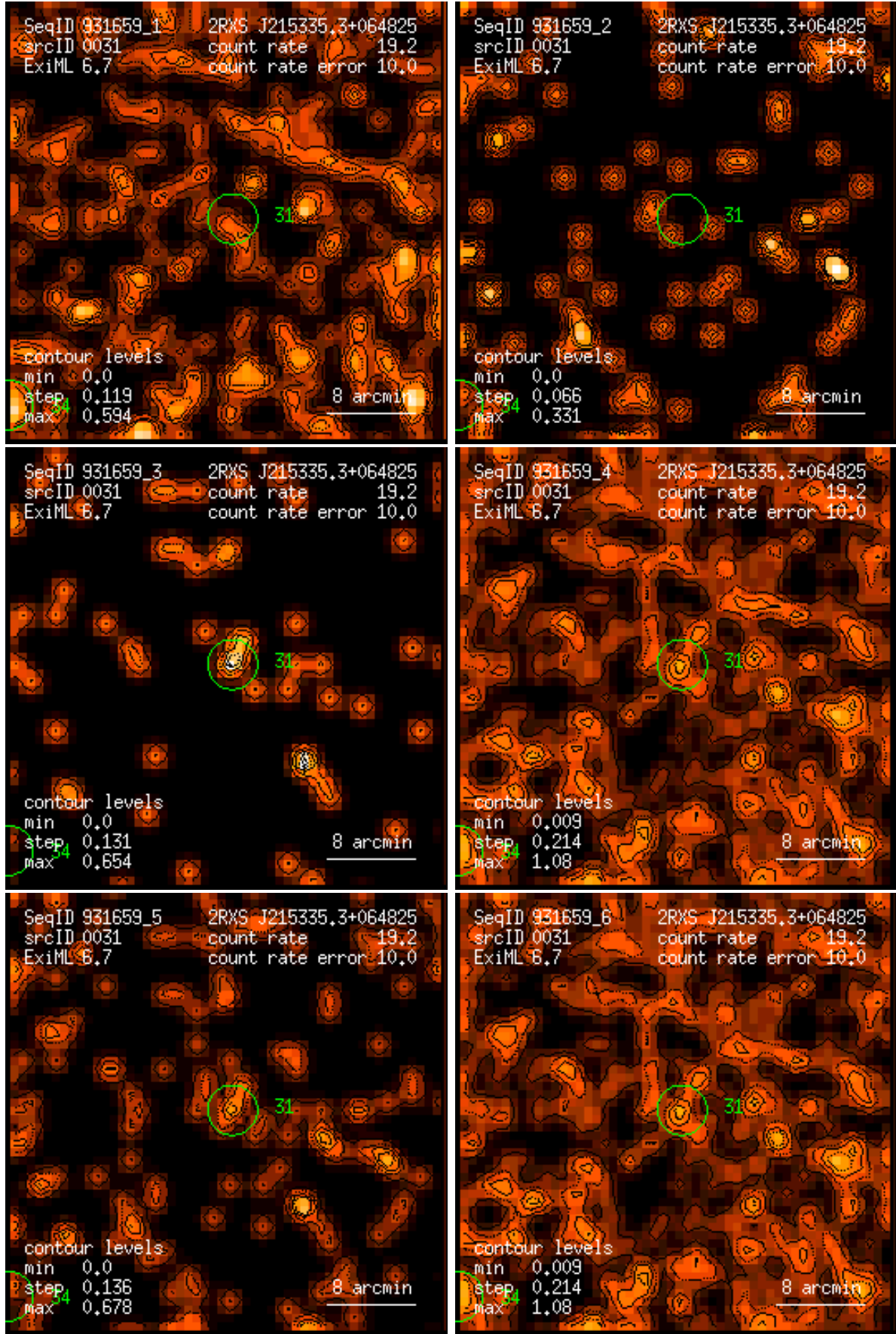
Figure 31: RASS 931659: detection 0031: band rate images, Gaussian filter: (1) PSPC channels 11 – 41, (2) 52 – 90, (3) 91 – 201, (4) 11 – 235, (5) 52 – 201, (6) 11 – 201. Broad band rates in counts/ks. Band rate contour levels in counts/ks/arcmin 2 .
