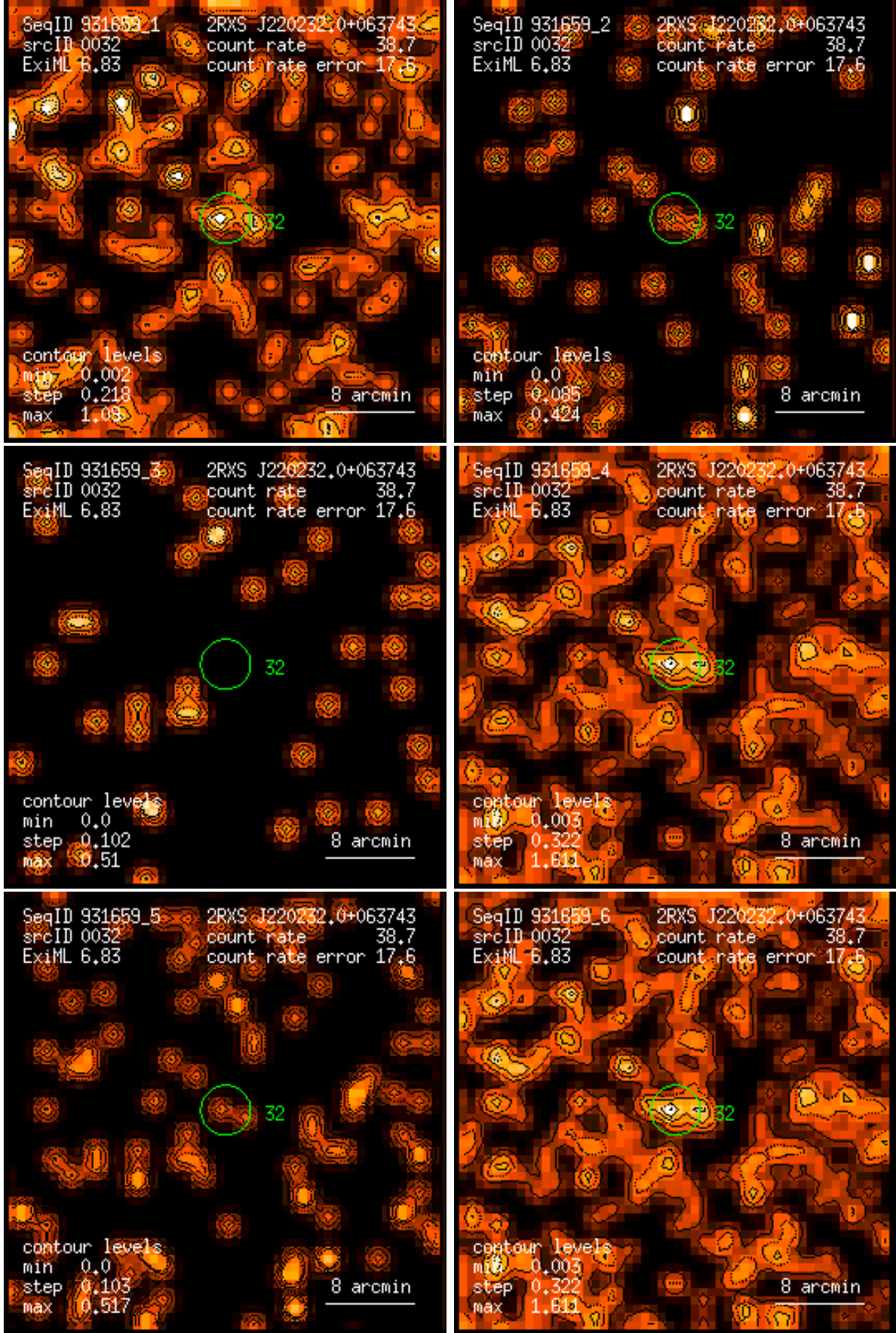
Figure 32: RASS 931659: detection 0032: band rate images, Gaussian filter: (1) PSPC channels 11 – 41, (2) 52 – 90, (3) 91 – 201, (4) 11 – 235, (5) 52 – 201, (6) 11 – 201. Broad band rates in counts/ks. Band rate contour levels in counts/ks/arcmin 2 .
