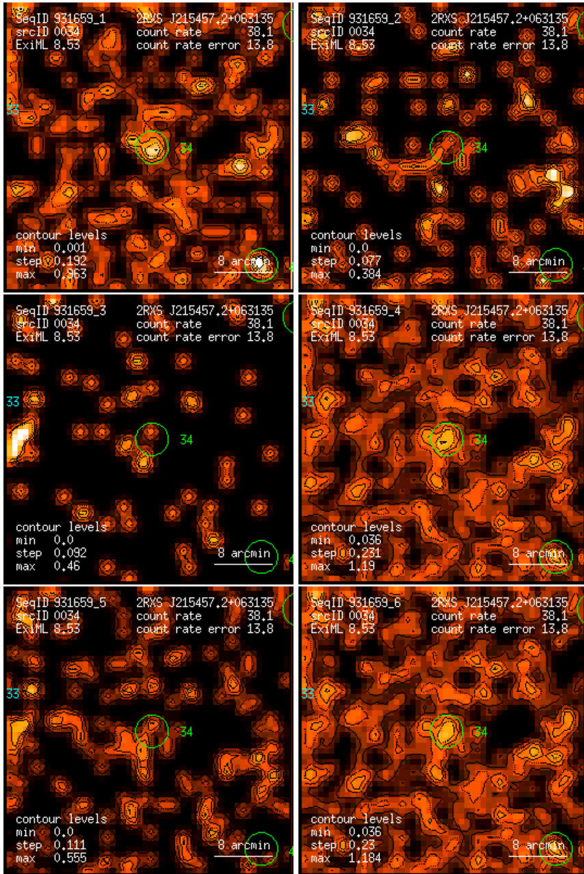
Figure 34: RASS 931659: detection 0034: band rate images, Gaussian filter: (1) PSPC channels 11 – 41, (2) 52 – 90, (3) 91 – 201, (4) 11 – 235, (5) 52 – 201, (6) 11 – 201. Broad band rates in counts/ks. Band rate contour levels in counts/ks/arcmin 2 .
