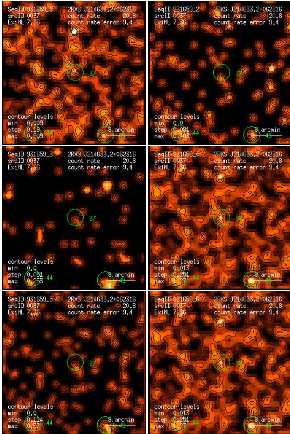
Figure 37: RASS 931659: detection 0037: band rate images, Gaussian filter: (1) PSPC channels 11 – 41, (2) 52 – 90, (3) 91 – 201, (4) 11 – 235, (5) 52 – 201, (6) 11 – 201. Broad band rates in counts/ks. Band rate contour levels in counts/ks/arcmin 2 .
