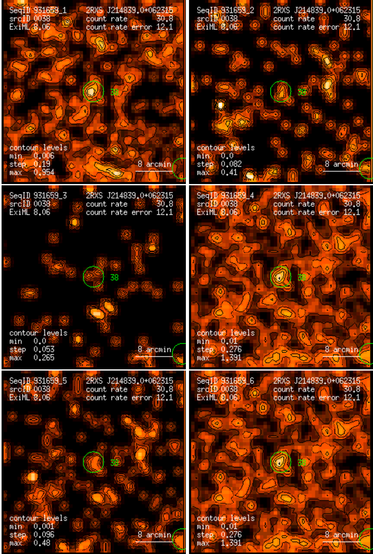
Figure 38: RASS 931659: detection 0038: band rate images, Gaussian filter: (1) PSPC channels 11 – 41, (2) 52 – 90, (3) 91 – 201, (4) 11 – 235, (5) 52 – 201, (6) 11 – 201. Broad band rates in counts/ks. Band rate contour levels in counts/ks/arcmin 2 .
