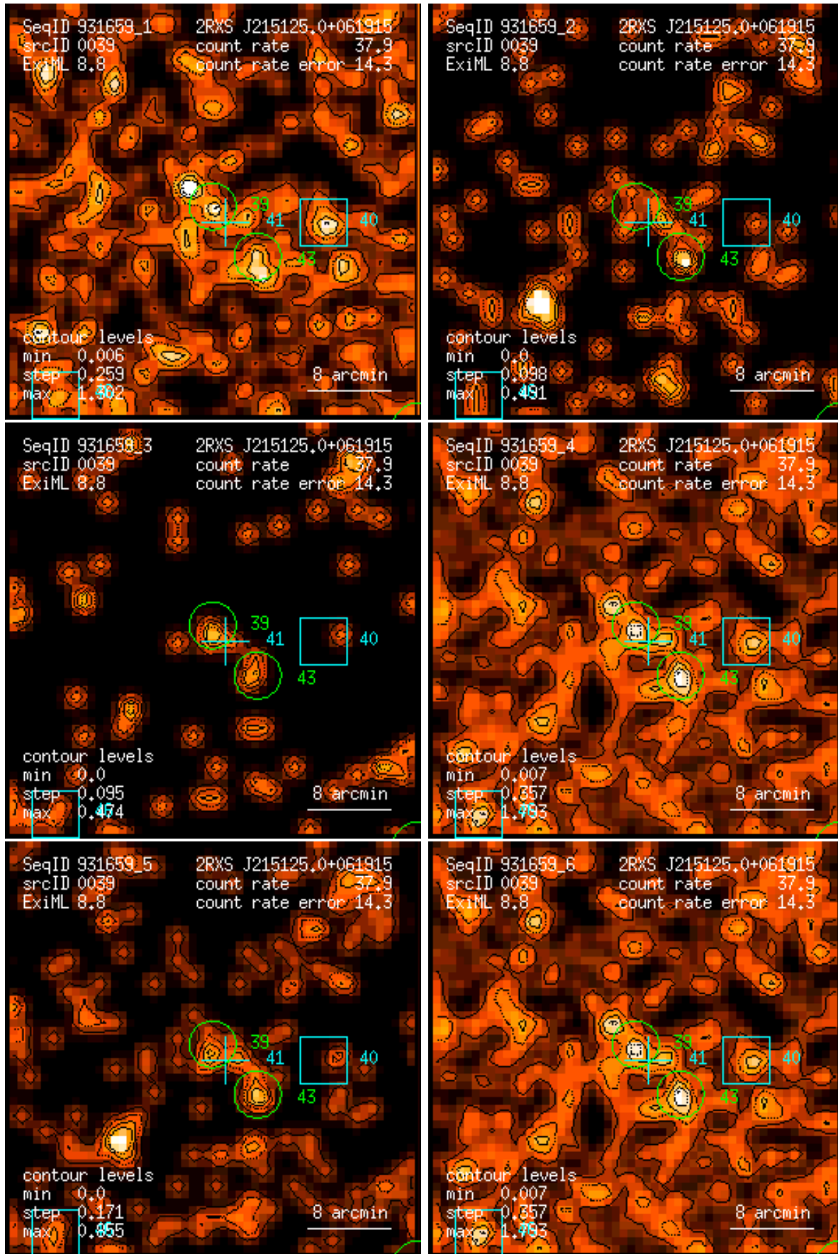
Figure 39: RASS 931659: detection 0039: band rate images, Gaussian filter: (1) PSPC channels 11 – 41, (2) 52 – 90, (3) 91 – 201, (4) 11 – 235, (5) 52 – 201, (6) 11 – 201. Broad band rates in counts/ks. Band rate contour levels in counts/ks/arcmin 2 .
