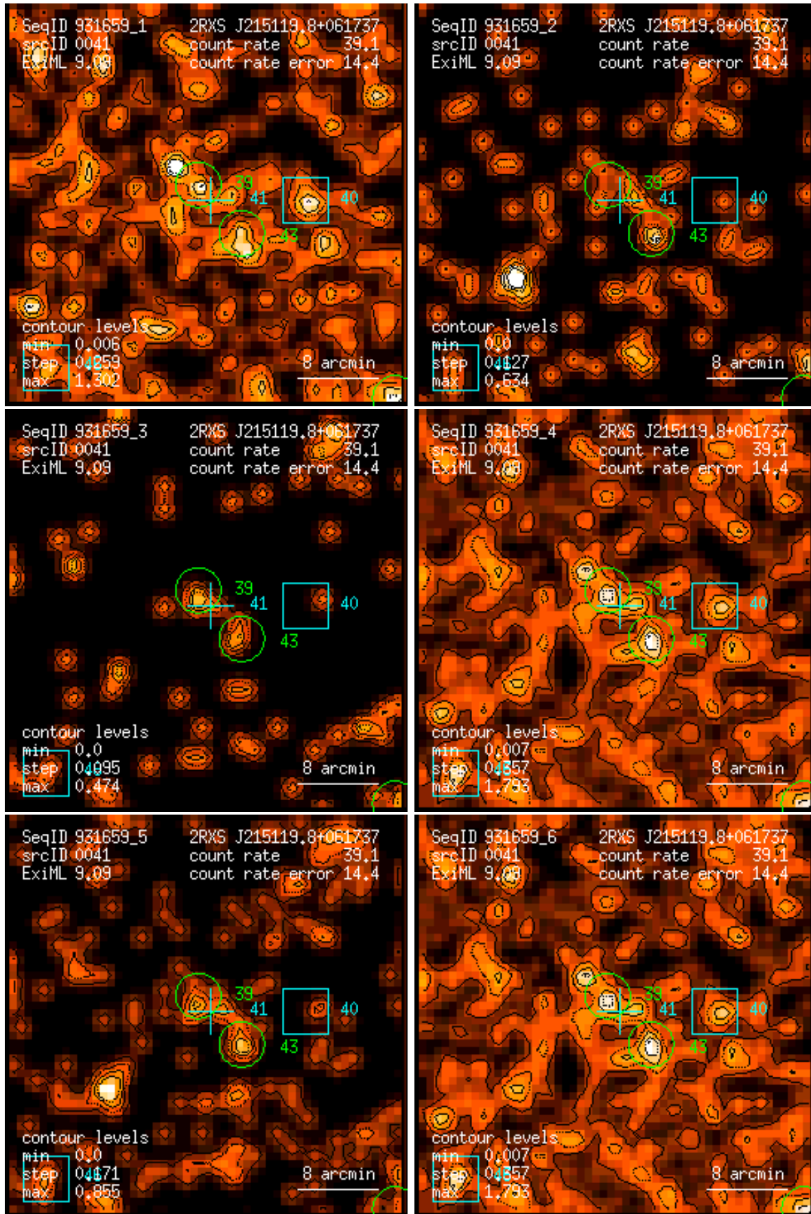
Figure 41: RASS 931659: detection 0041: band rate images, Gaussian filter: (1) PSPC channels 11 – 41, (2) 52 – 90, (3) 91 – 201, (4) 11 – 235, (5) 52 – 201, (6) 11 – 201. Broad band rates in counts/ks. Band rate contour levels in counts/ks/arcmin 2 .
