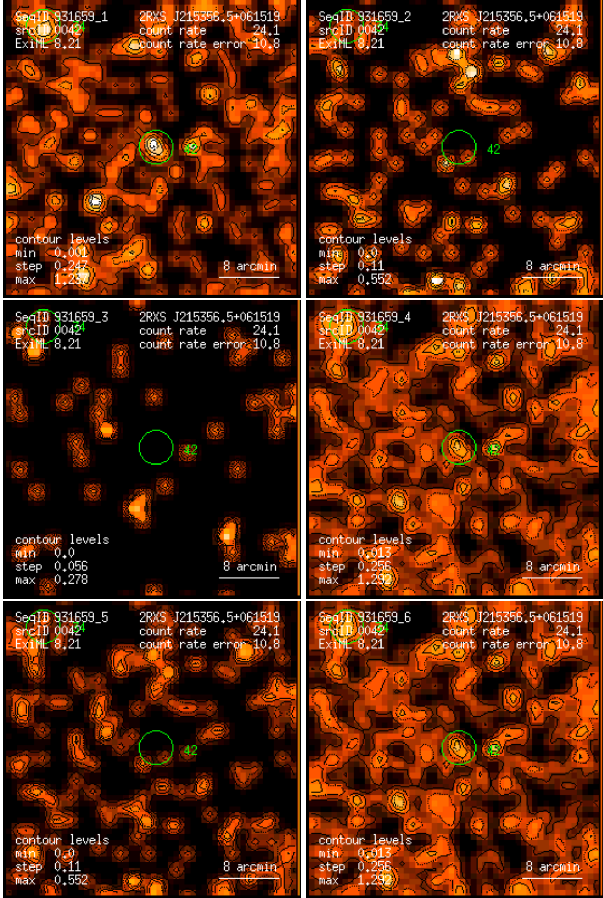
Figure 42: RASS 931659: detection 0042: band rate images, Gaussian filter: (1) PSPC channels 11 – 41, (2) 52 – 90, (3) 91 – 201, (4) 11 – 235, (5) 52 – 201, (6) 11 – 201. Broad band rates in counts/ks. Band rate contour levels in counts/ks/arcmin 2 .
