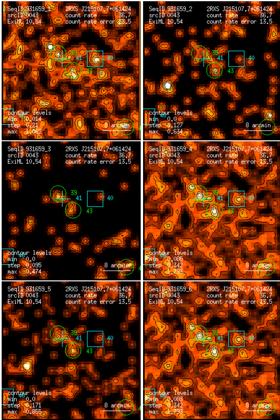
Figure 43: RASS 931659: detection 0043: band rate images, Gaussian filter: (1) PSPC channels 11 – 41, (2) 52 – 90, (3) 91 – 201, (4) 11 – 235, (5) 52 – 201, (6) 11 – 201. Broad band rates in counts/ks. Band rate contour levels in counts/ks/arcmin 2 .
