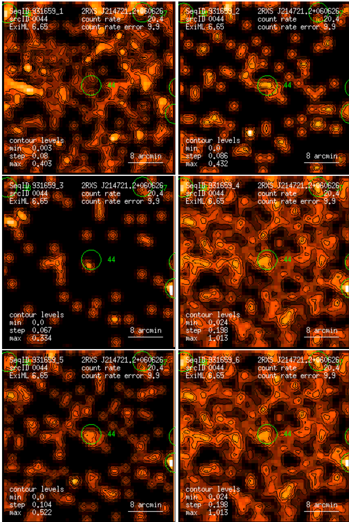
Figure 44: RASS 931659: detection 0044: band rate images, Gaussian filter: (1) PSPC channels 11 – 41, (2) 52 – 90, (3) 91 – 201, (4) 11 – 235, (5) 52 – 201, (6) 11 – 201. Broad band rates in counts/ks. Band rate contour levels in counts/ks/arcmin 2 .
