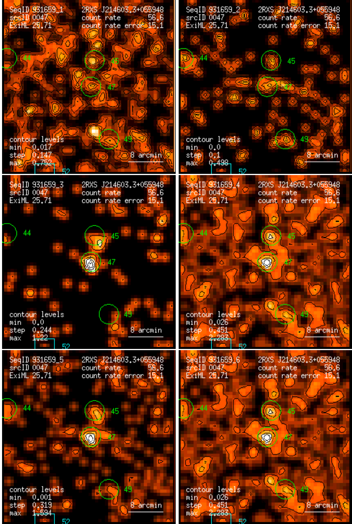
Figure 47: RASS 931659: detection 0047: band rate images, Gaussian filter: (1) PSPC channels 11 – 41, (2) 52 – 90, (3) 91 – 201, (4) 11 – 235, (5) 52 – 201, (6) 11 – 201. Broad band rates in counts/ks. Band rate contour levels in counts/ks/arcmin 2 .
