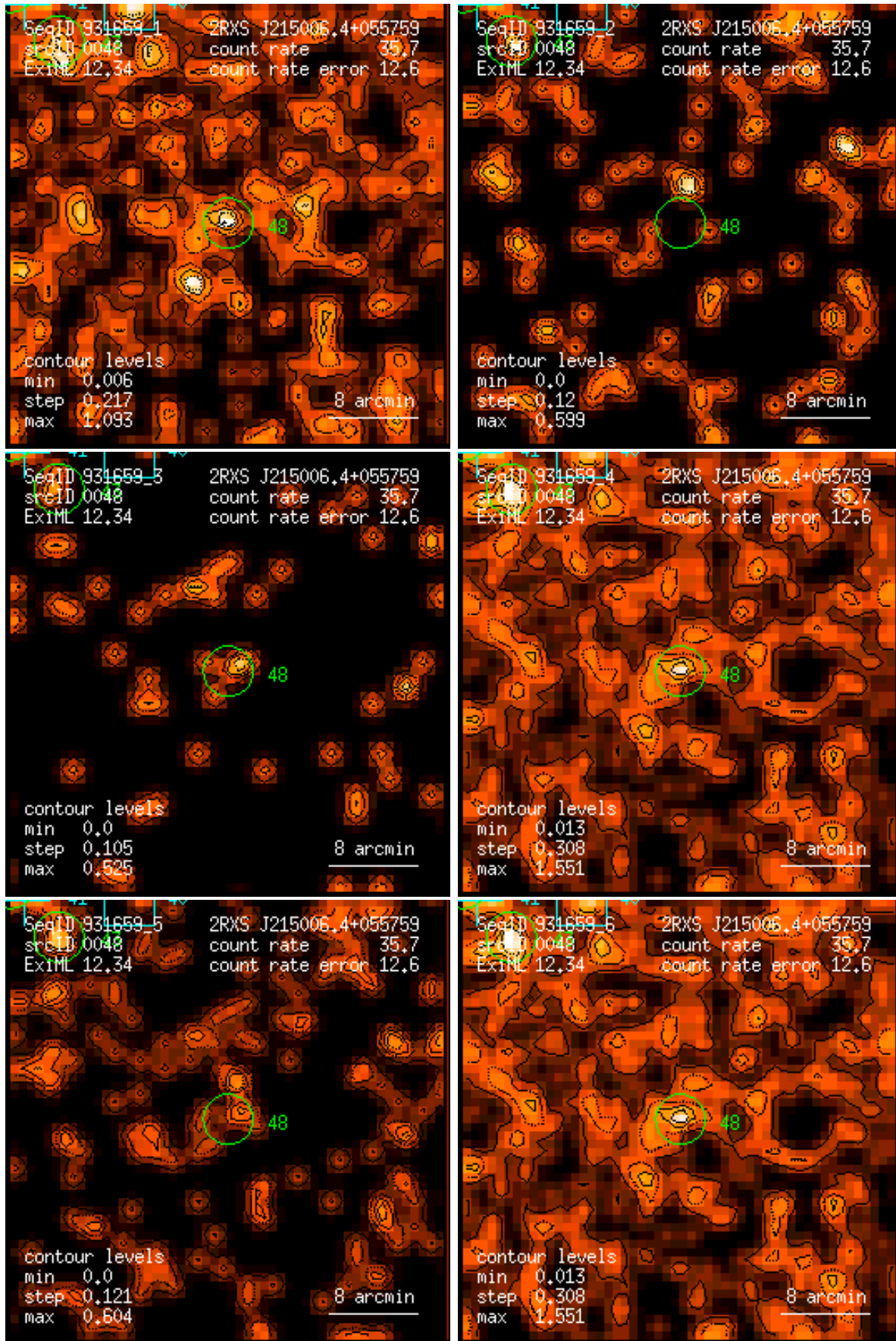
Figure 48: RASS 931659: detection 0048: band rate images, Gaussian filter: (1) PSPC channels 11 – 41, (2) 52 – 90, (3) 91 – 201, (4) 11 – 235, (5) 52 – 201, (6) 11 – 201. Broad band rates in counts/ks. Band rate contour levels in counts/ks/arcmin 2 .
