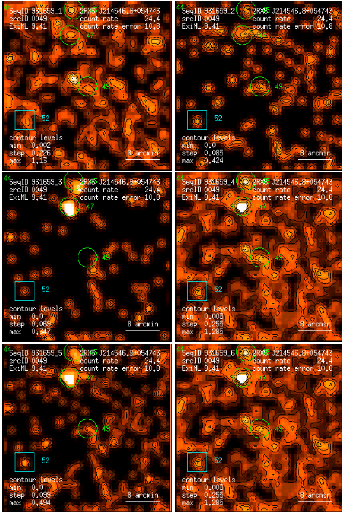
Figure 49: RASS 931659: detection 0049: band rate images, Gaussian filter: (1) PSPC channels 11 – 41, (2) 52 – 90, (3) 91 – 201, (4) 11 – 235, (5) 52 – 201, (6) 11 – 201. Broad band rates in counts/ks. Band rate contour levels in counts/ks/arcmin 2 .
