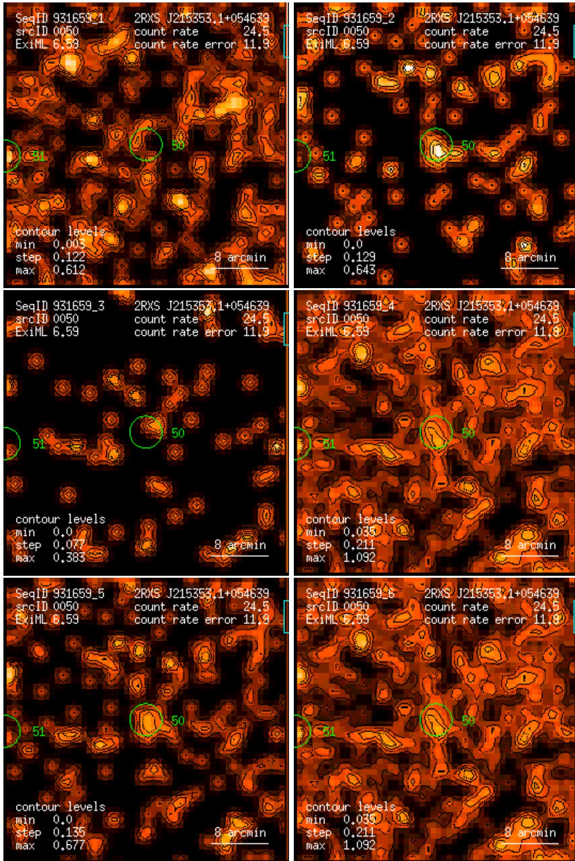
Figure 50: RASS 931659: detection 0050: band rate images, Gaussian filter: (1) PSPC channels 11 – 41, (2) 52 – 90, (3) 91 – 201, (4) 11 – 235, (5) 52 – 201, (6) 11 – 201. Broad band rates in counts/ks. Band rate contour levels in counts/ks/arcmin 2 .
