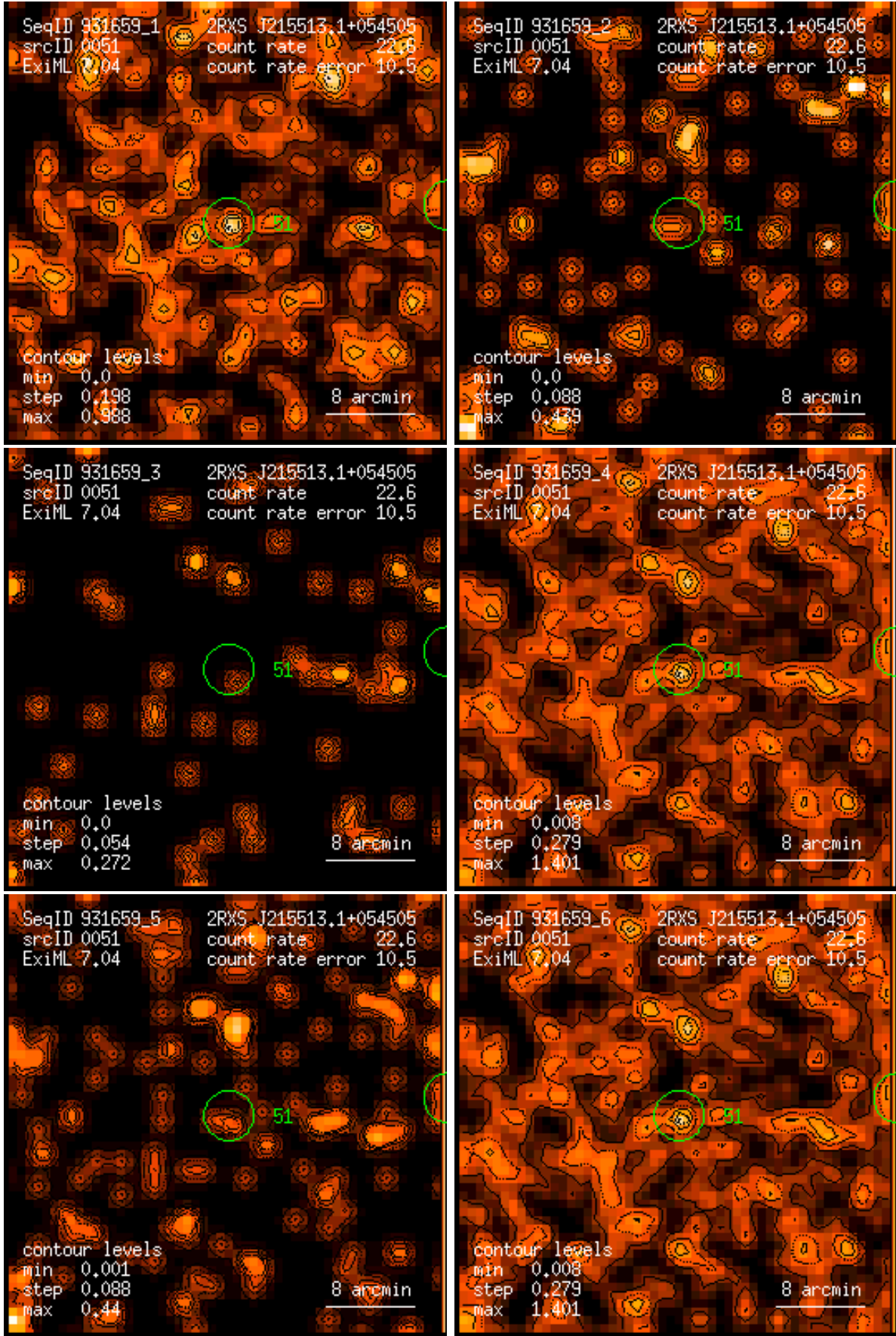
Figure 51: RASS 931659: detection 0051: band rate images, Gaussian filter: (1) PSPC channels 11 – 41, (2) 52 – 90, (3) 91 – 201, (4) 11 – 235, (5) 52 – 201, (6) 11 – 201. Broad band rates in counts/ks. Band rate contour levels in counts/ks/arcmin 2 .
