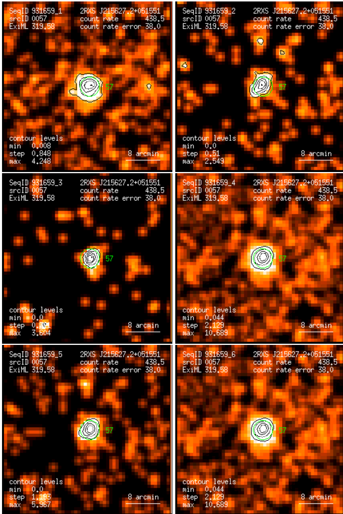
Figure 57: RASS 931659: detection 0057: band rate images, Gaussian filter: (1) PSPC channels 11 – 41, (2) 52 – 90, (3) 91 – 201, (4) 11 – 235, (5) 52 – 201, (6) 11 – 201. Broad band rates in counts/ks. Band rate contour levels in counts/ks/arcmin 2 .
