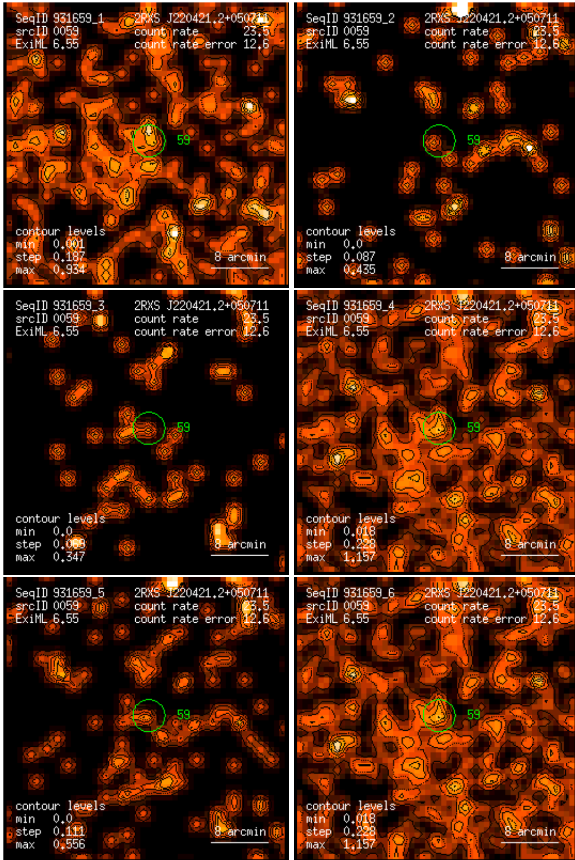
Figure 59: RASS 931659: detection 0059: band rate images, Gaussian filter: (1) PSPC channels 11 – 41, (2) 52 – 90, (3) 91 – 201, (4) 11 – 235, (5) 52 – 201, (6) 11 – 201. Broad band rates in counts/ks. Band rate contour levels in counts/ks/arcmin 2 .
