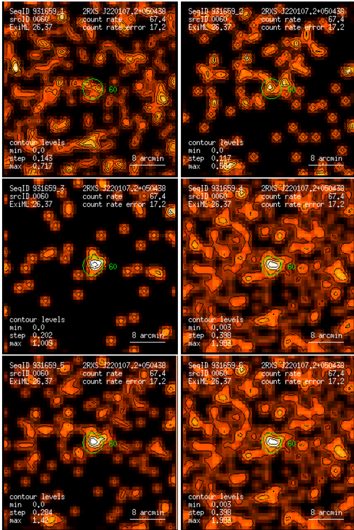
Figure 60: RASS 931659: detection 0060: band rate images, Gaussian filter: (1) PSPC channels 11 – 41, (2) 52 – 90, (3) 91 – 201, (4) 11 – 235, (5) 52 – 201, (6) 11 – 201. Broad band rates in counts/ks. Band rate contour levels in counts/ks/arcmin 2 .
