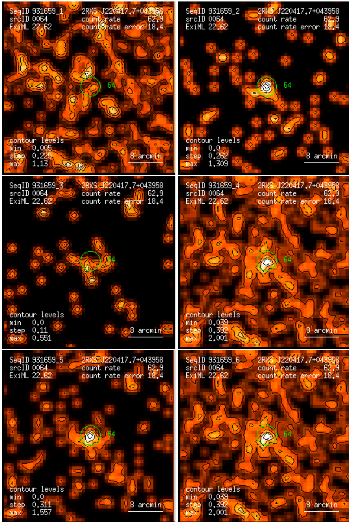
Figure 64: RASS 931659: detection 0064: band rate images, Gaussian filter: (1) PSPC channels 11 – 41, (2) 52 – 90, (3) 91 – 201, (4) 11 – 235, (5) 52 – 201, (6) 11 – 201. Broad band rates in counts/ks. Band rate contour levels in counts/ks/arcmin 2 .
