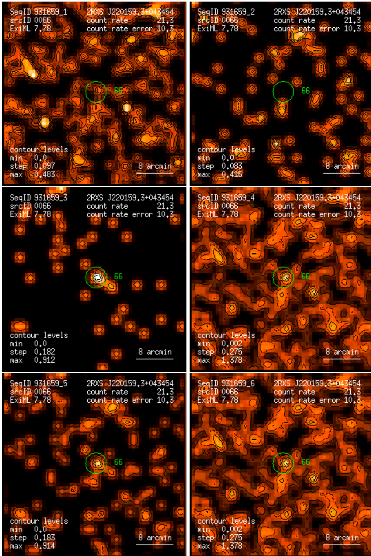
Figure 66: RASS 931659: detection 0066: band rate images, Gaussian filter: (1) PSPC channels 11 – 41, (2) 52 – 90, (3) 91 – 201, (4) 11 – 235, (5) 52 – 201, (6) 11 – 201. Broad band rates in counts/ks. Band rate contour levels in counts/ks/arcmin 2 .
