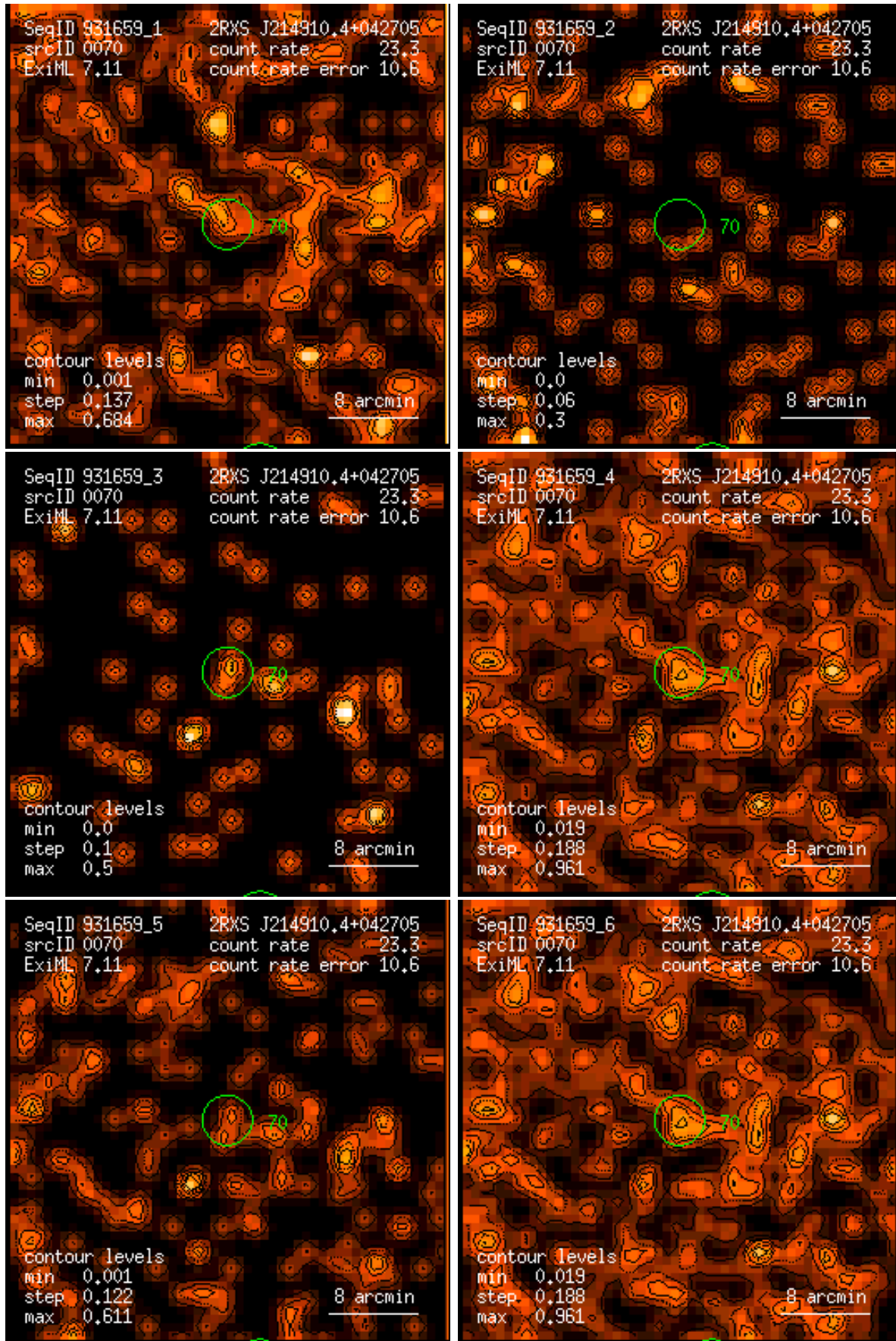
Figure 70: RASS 931659: detection 0070: band rate images, Gaussian filter: (1) PSPC channels 11 – 41, (2) 52 – 90, (3) 91 – 201, (4) 11 – 235, (5) 52 – 201, (6) 11 – 201. Broad band rates in counts/ks. Band rate contour levels in counts/ks/arcmin 2 .
