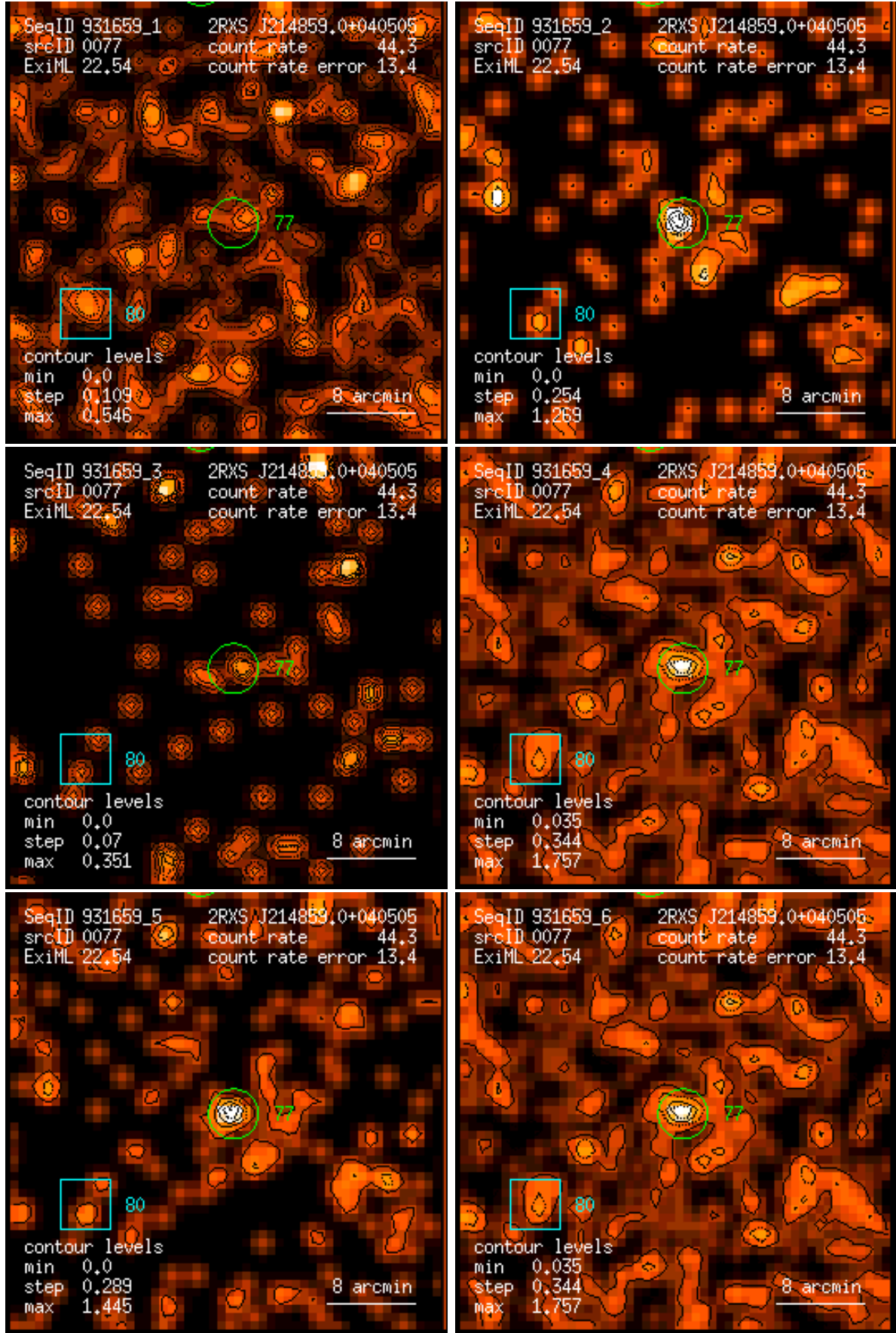
Figure 77: RASS 931659: detection 0077: band rate images, Gaussian filter: (1) PSPC channels 11 – 41, (2) 52 – 90, (3) 91 – 201, (4) 11 – 235, (5) 52 – 201, (6) 11 – 201. Broad band rates in counts/ks. Band rate contour levels in counts/ks/arcmin 2 .
