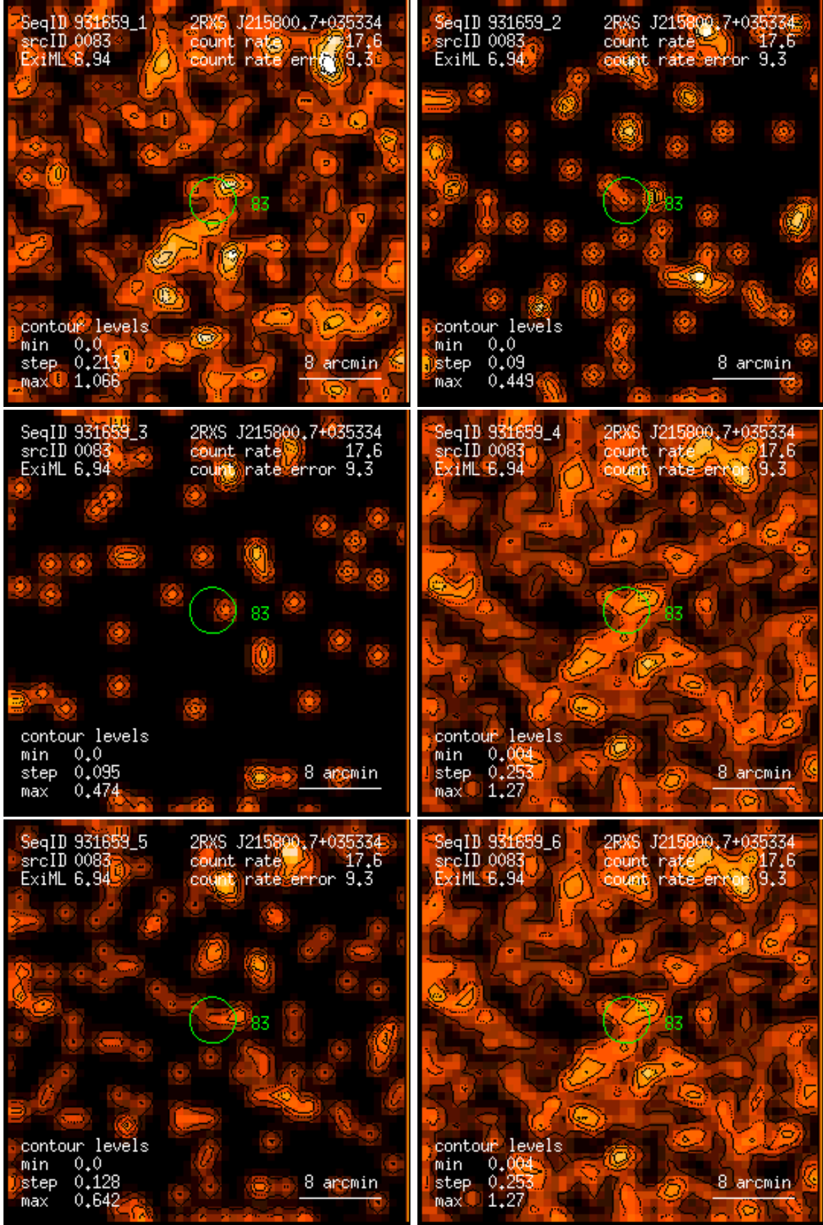
Figure 83: RASS 931659: detection 0083: band rate images, Gaussian filter: (1) PSPC channels 11 – 41, (2) 52 – 90, (3) 91 – 201, (4) 11 – 235, (5) 52 – 201, (6) 11 – 201. Broad band rates in counts/ks. Band rate contour levels in counts/ks/arcmin 2 .
