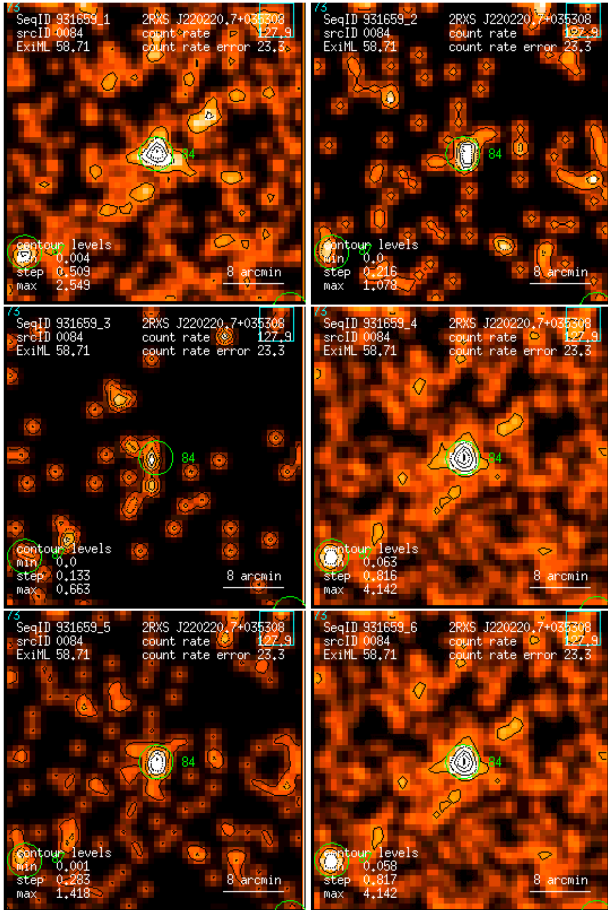
Figure 84: RASS 931659: detection 0084: band rate images, Gaussian filter: (1) PSPC channels 11 – 41, (2) 52 – 90, (3) 91 – 201, (4) 11 – 235, (5) 52 – 201, (6) 11 – 201. Broad band rates in counts/ks. Band rate contour levels in counts/ks/arcmin 2 .
