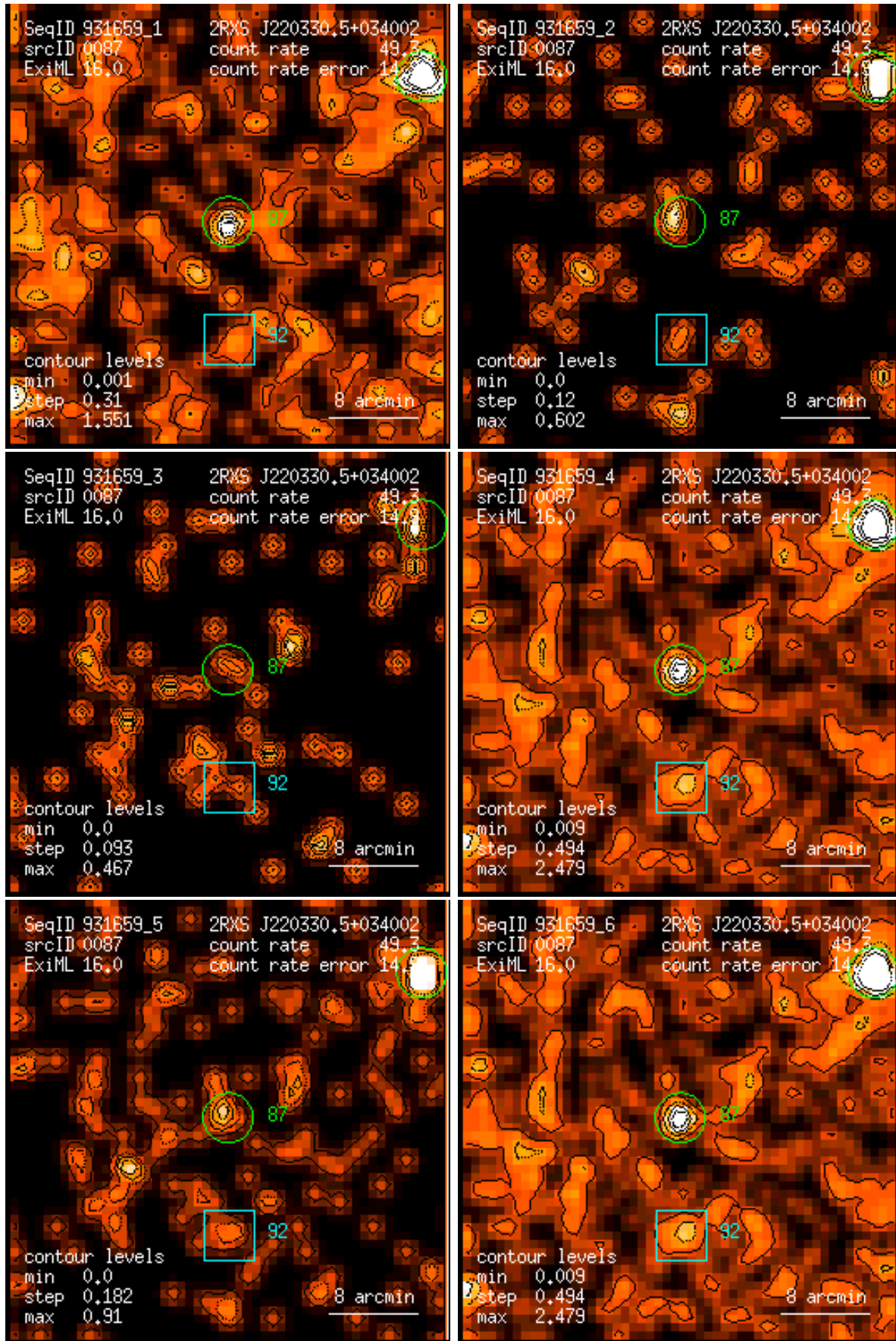
Figure 87: RASS 931659: detection 0087: band rate images, Gaussian filter: (1) PSPC channels 11 – 41, (2) 52 – 90, (3) 91 – 201, (4) 11 – 235, (5) 52 – 201, (6) 11 – 201. Broad band rates in counts/ks. Band rate contour levels in counts/ks/arcmin 2 .
