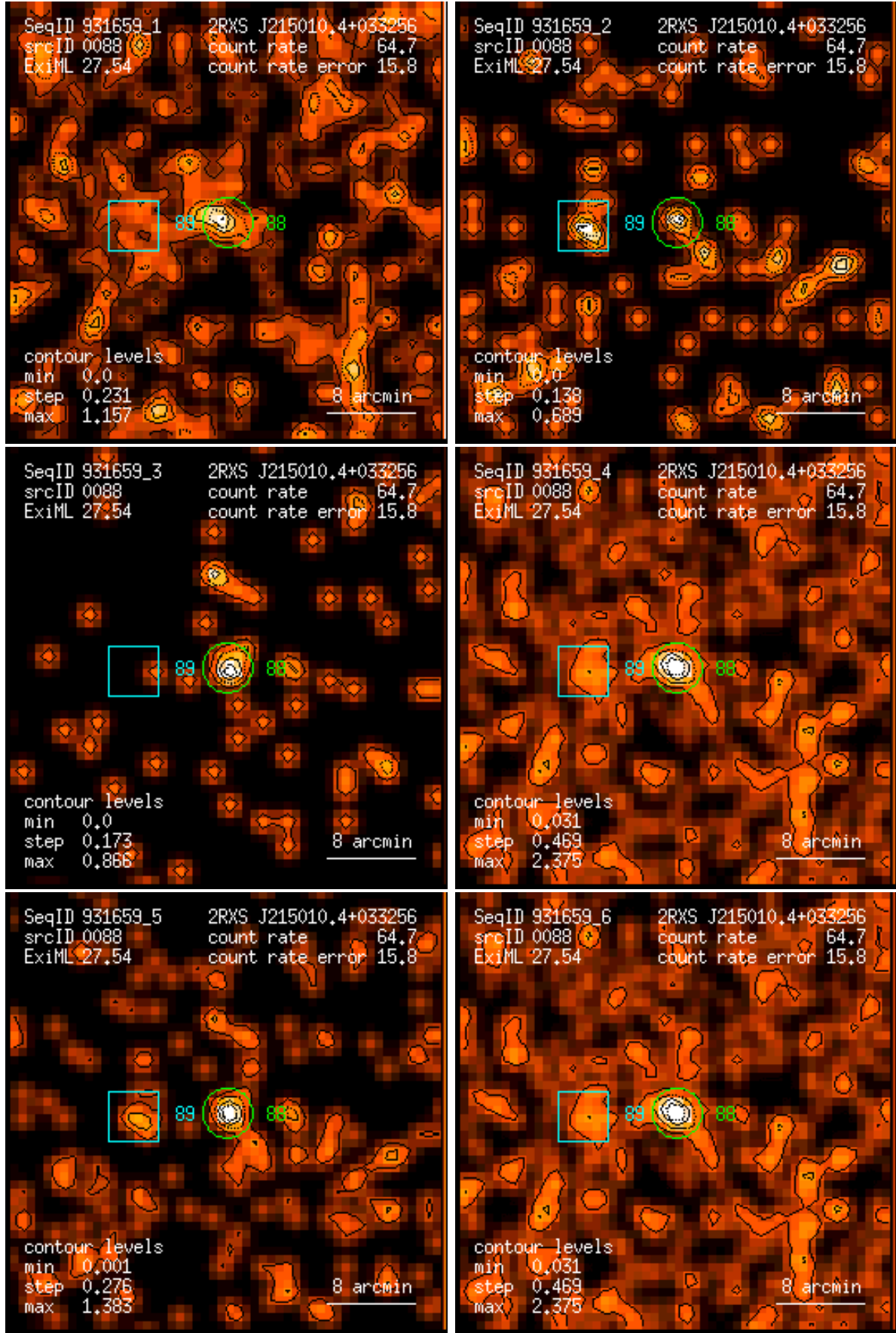
Figure 88: RASS 931659: detection 0088: band rate images, Gaussian filter: (1) PSPC channels 11 – 41, (2) 52 – 90, (3) 91 – 201, (4) 11 – 235, (5) 52 – 201, (6) 11 – 201. Broad band rates in counts/ks. Band rate contour levels in counts/ks/arcmin 2 .
