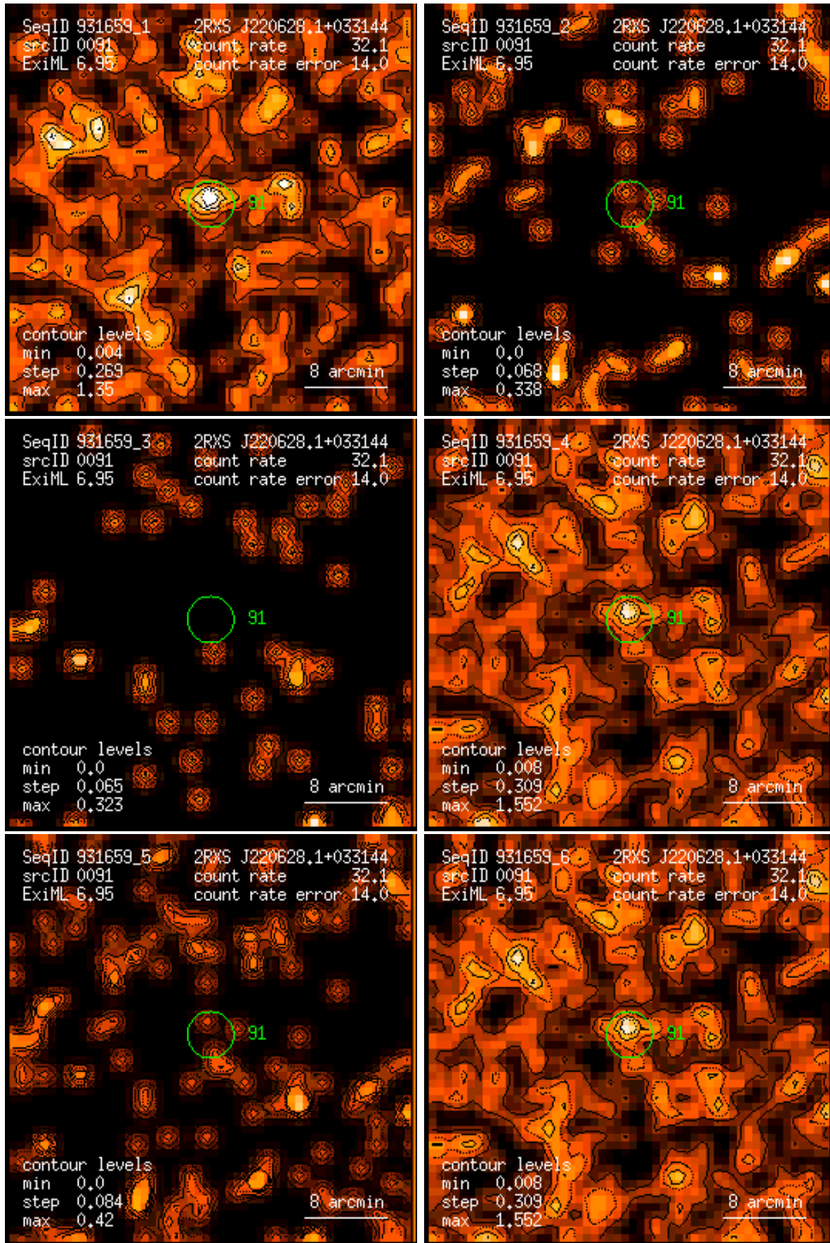
Figure 91: RASS 931659: detection 0091: band rate images, Gaussian filter: (1) PSPC channels 11 – 41, (2) 52 – 90, (3) 91 – 201, (4) 11 – 235, (5) 52 – 201, (6) 11 – 201. Broad band rates in counts/ks. Band rate contour levels in counts/ks/arcmin 2 .
